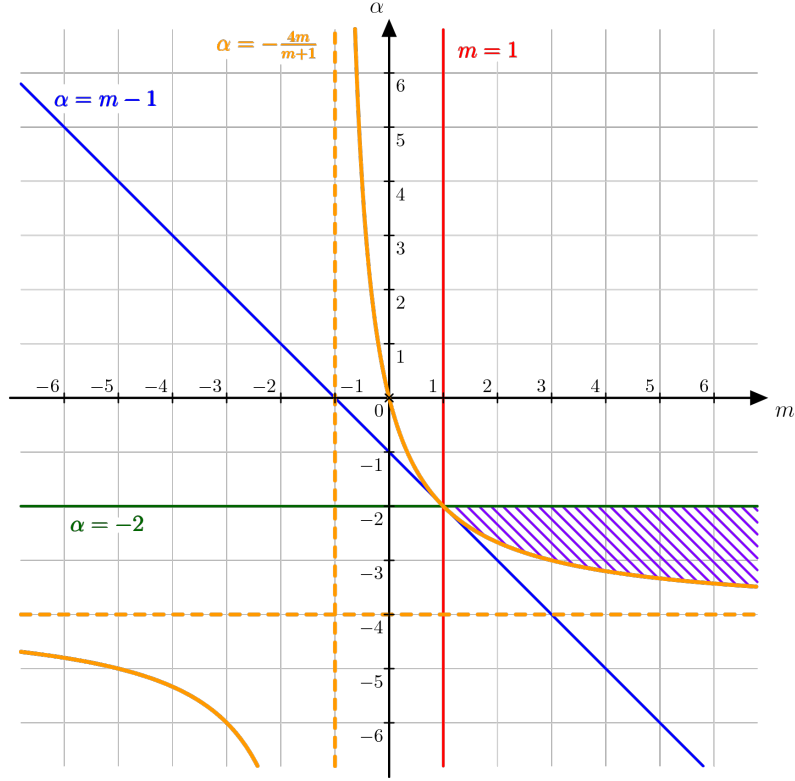
Fig. 3.3: Solution of the system (3.42)
