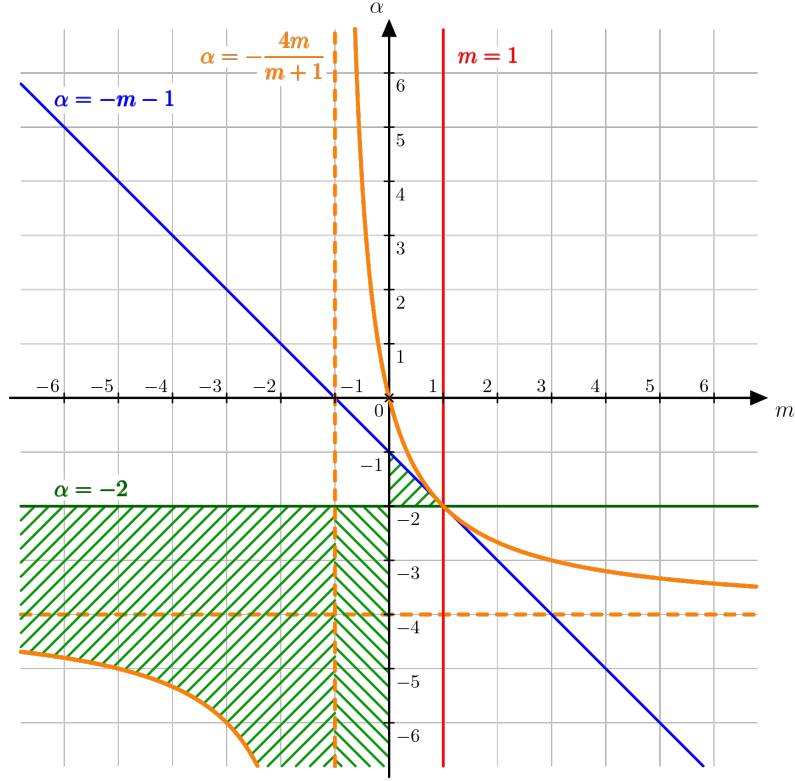
Fig. 3.4: Solution of the system (3.43)
