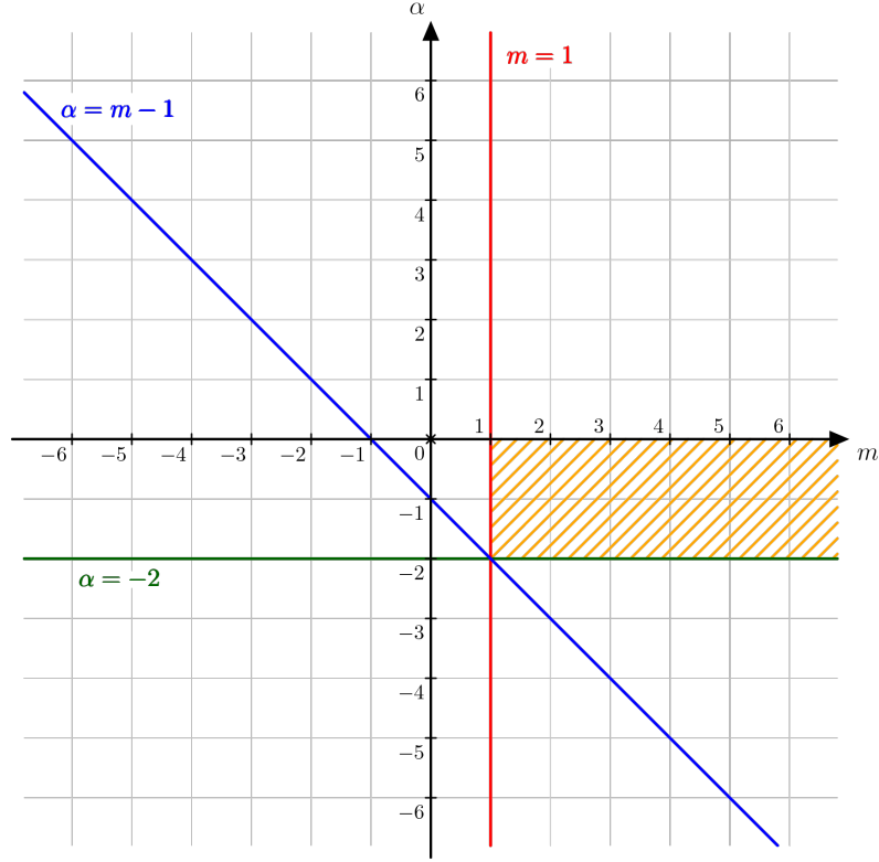
Fig. 3.1: Solution of the system (3.38)
