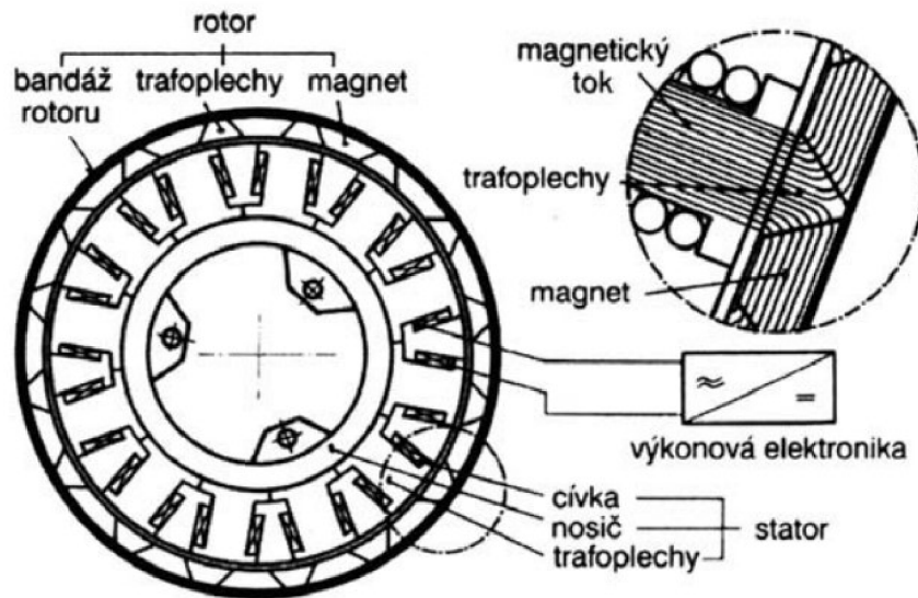
Obr. 1.2 Elektromotor magnet-motor
