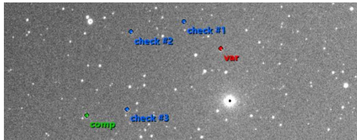
Figure 20: Chosen stars – variable, comparison, and check-stars.
