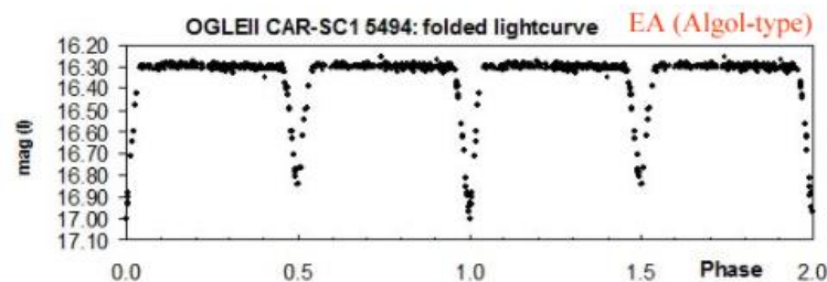
Figure 6a: Light curve of an EA-type binary star. Modified. [28]
