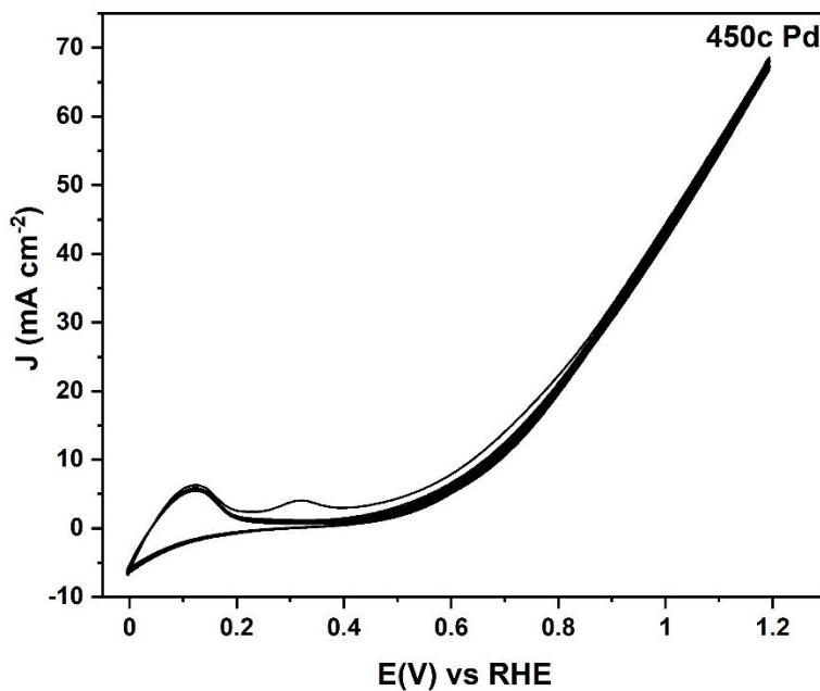
Figure 2.A.7. Cyclic voltammogram for the TNT layer decorated with 450c Pd ALD cycles, recorded for 22 cycles in 1M KOH + 1M CH 3 OH.
