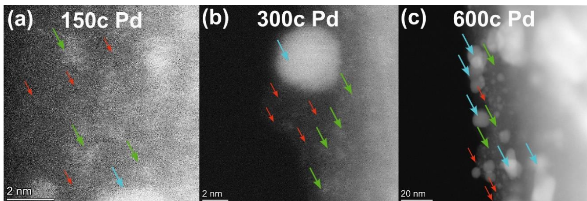
Figure 3.A.2. (a) CP 150c Pd; (b) CP 300c Pd and (c) 600c Pd HAADF-STEM images. Arrow marks in red indicate SAs, green indicates atomic clusters and cyan indicate larger NPs.
