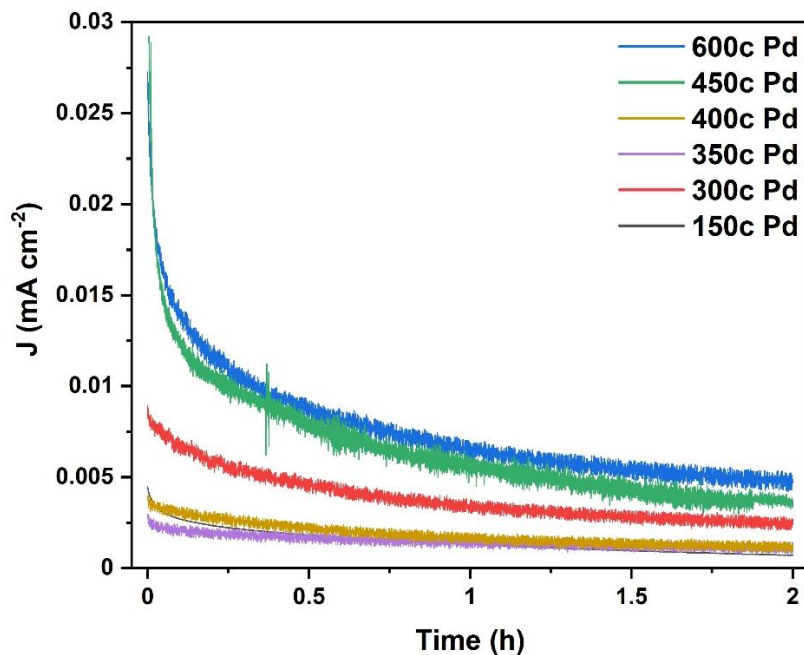
Figure 2.A.6. Chrono-amperometric curves recorded to evaluate the stability of Pd decorated Ti foils with different N_{ALD} = 150, 300, 350, 400, 450, and 600 , recorded in 1M KOH + 1M CH 3 OH at 0.9V for 2 h.
