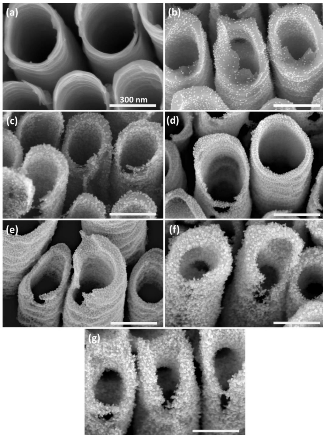
Figure 2.1. SEM top views of 5 \mu\text{m} thick TNT layers decorated with Pd NPs using different N_{\text{ALD}} : (a) 0, (b) 150, (c) 300, (d) 350, (e) 400, (f) 450, (g) 600. The scale bars in all images represent 300 nm.
