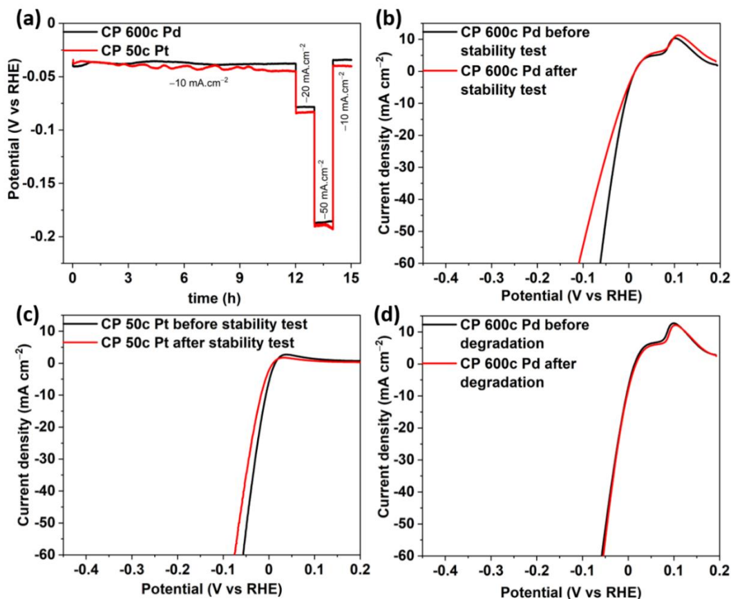
Figure 3.5. Stability measurement: a) stricase chronopotentiometry ; b) LSV before and after stability test for CP 600c Pd; c) LSV before and after stability test for CP 50c Pt; d) LSV before and after degradation test for CP 600c Pd.
