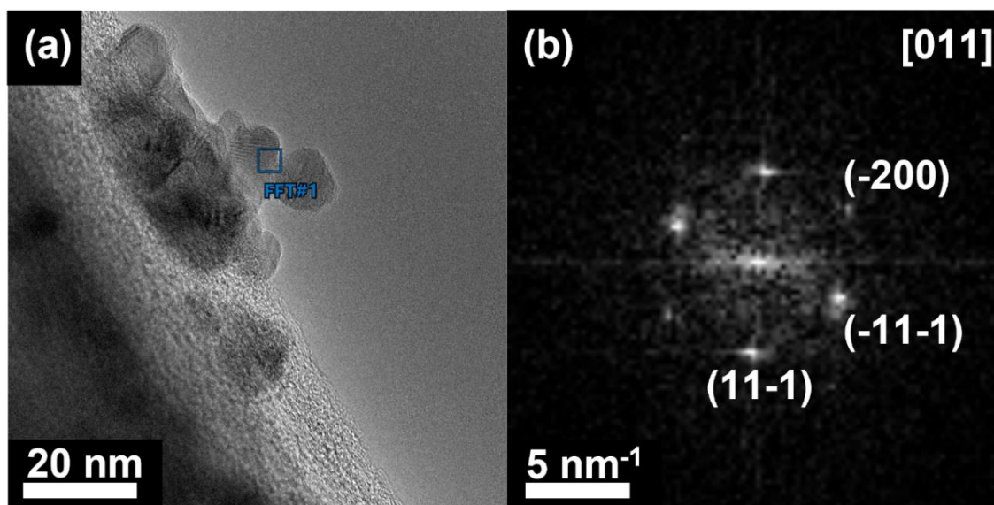
Figure 3.A.10. (a) HR TEM image for CP 600c Pd after stability measurements; (b) FFT analysis corresponding to a blue rectangle in (a).
