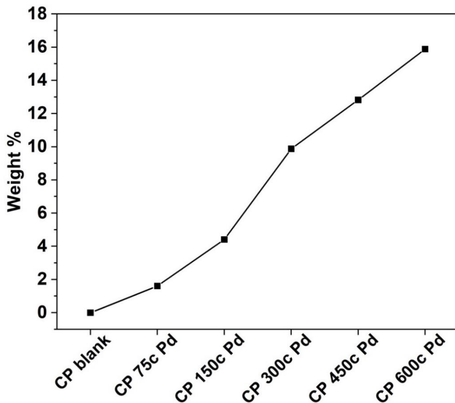
Figure 3.A.7. The weight percent of the loaded Pd on the carbon substrate analysed by inductive coupled plasma atomic emission spectroscopy (ICP-OES). The connecting line is used for eye guidance.
