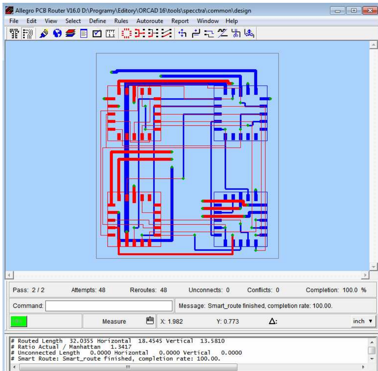
Obr. 3.13 Autorouter SPECCTRA for OrCAD
