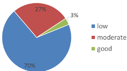
Fig. 11A. Quantitative ratio of solo howls in the HVM data set based on the quality of a recorded signal: low, moderate and good.
