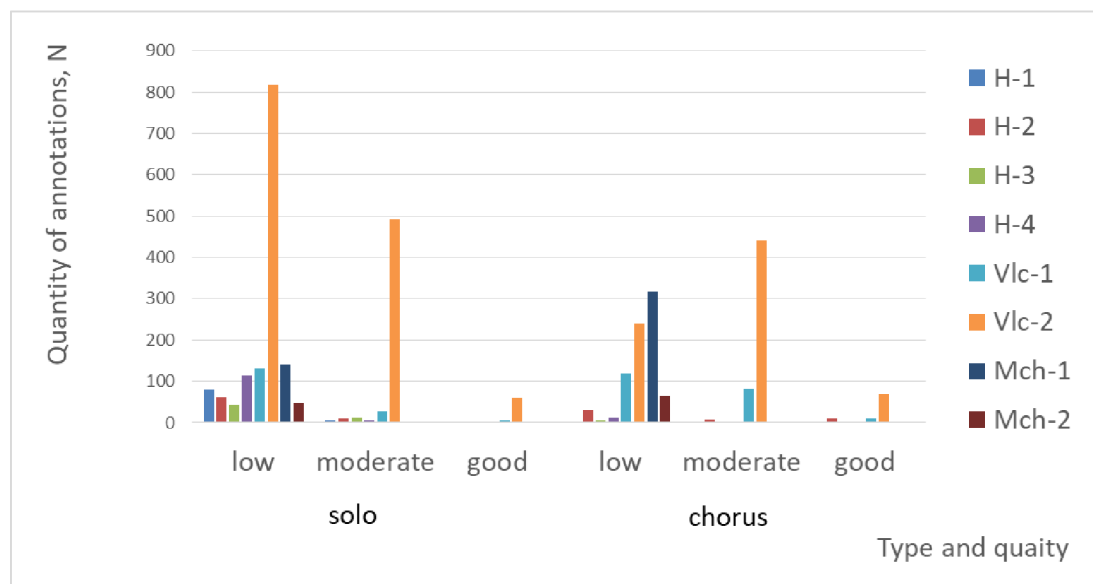
Fig.13. Quantity of annotations of low, moderate and high quality recorded solo and chorus wolf howls in eight batches of recordings: H - Hohwald, Vlc - Vlčinec, Mch - Mechov.
