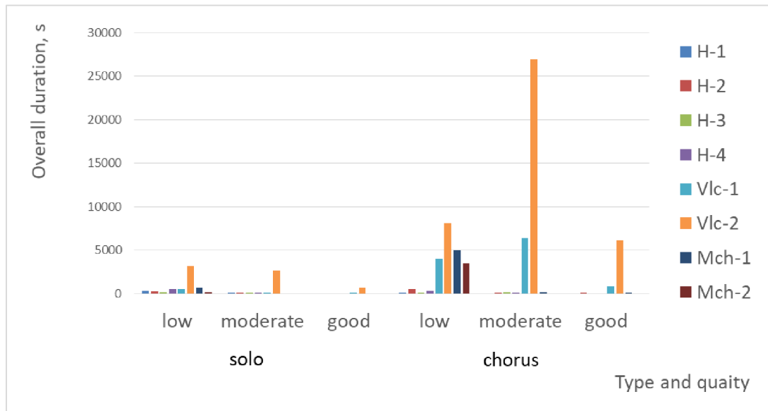
Fig.14. Overall duration of annotations of low, moderate and high quality recorded solo and chorus wolf howls in eight batches of recordings: H - Hohwald, Vlc - Vlčinec, Mch - Mechov.
