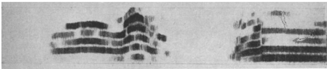
Fig 2. A spectrogram of a wolf signal received in the middle of the 20th century (Koenig et al., 1946).
