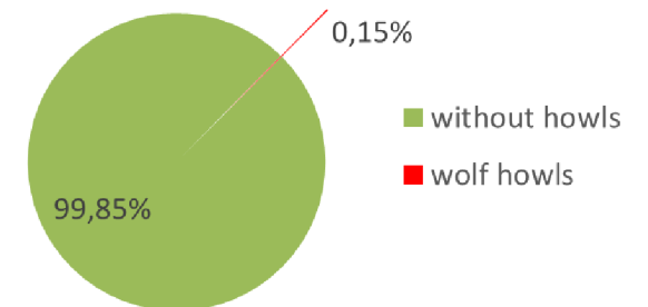
Fig. 7. Ratio of overall duration of wolf howls and time without howling in the HVM recordings.
