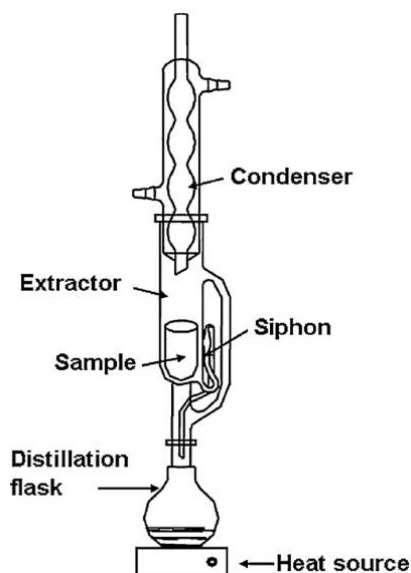
Figure 7: Conventional Soxhlet apparatus
