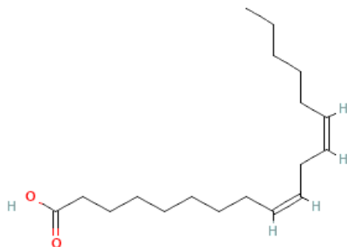
Figure 1: Chemical structure of linoleic acid
