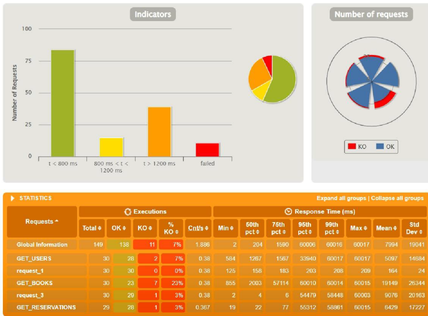
Figure 4.11: Results for test data: 2000 users, 4000 reservations, 8000 books, 200 actors - Micro-naut [2]
