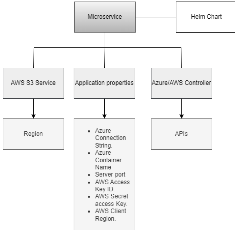
Figure 5.2: Microservice Composition
