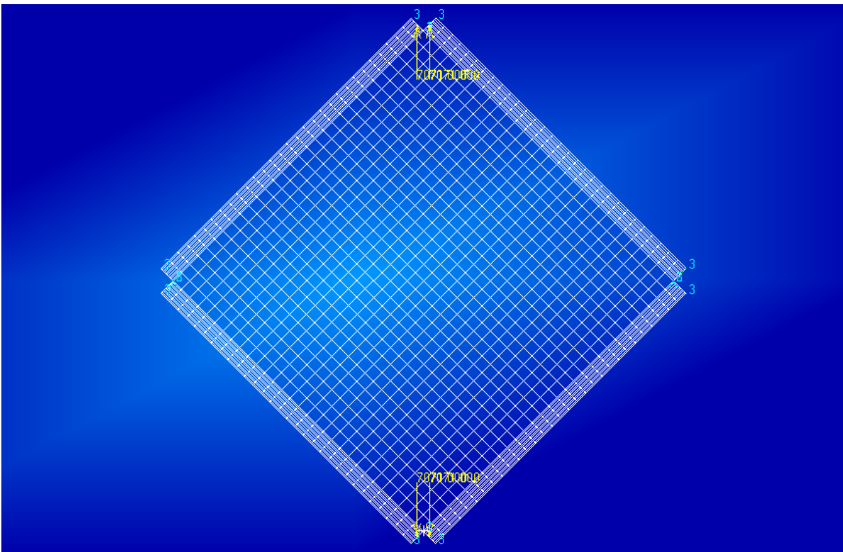
Figure 6. Loads and displacements representation for the first approach model.
