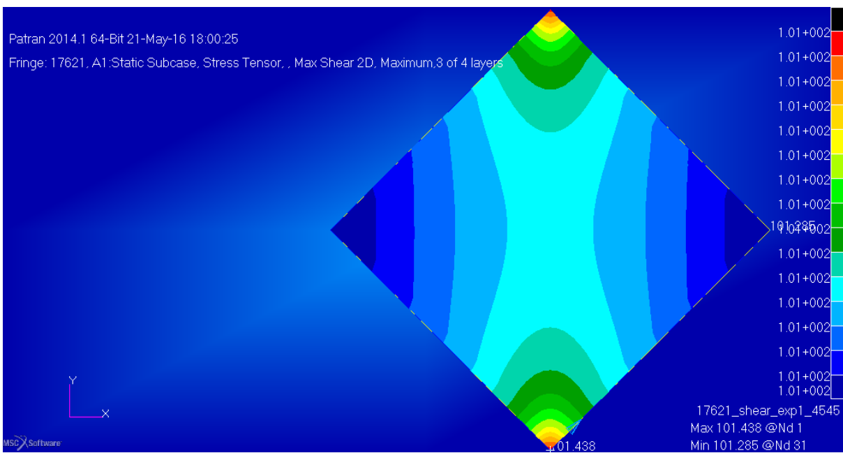
Figure 18. Graphic representation of stress in plate, load case F_{sim13} .
