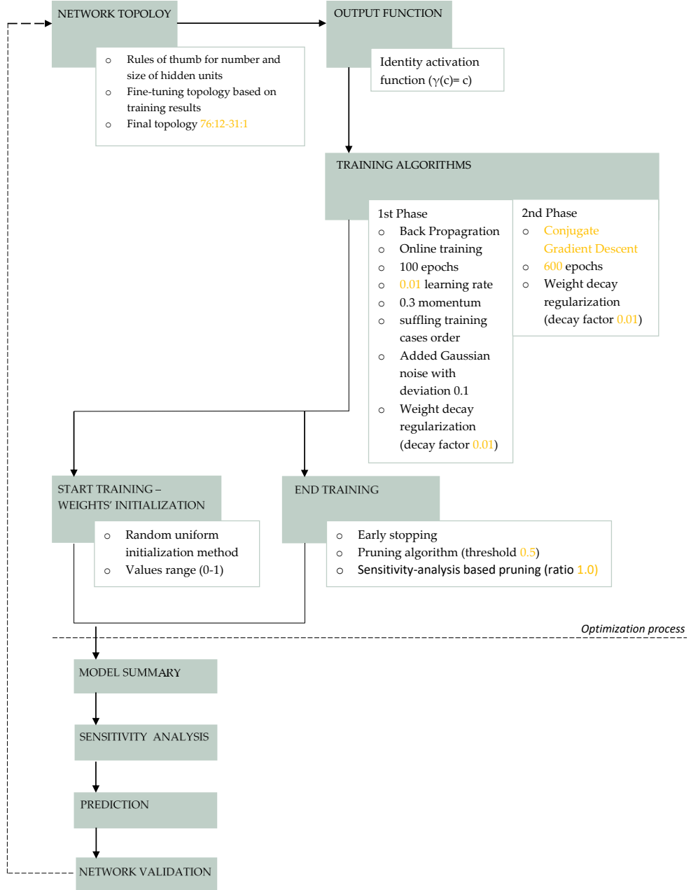
Figure 3. Flowchart of MLP network training.
