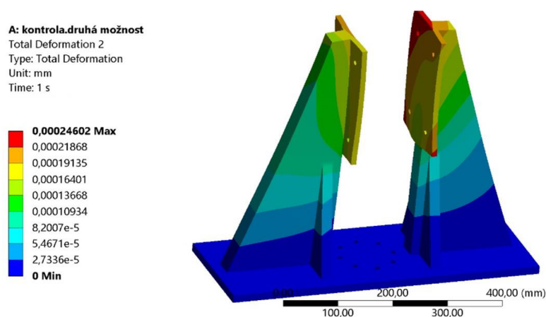
Obr. 4-11 Deformace ve stojanu
