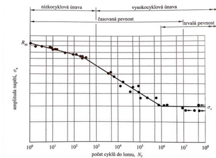
Obr. 2-4 Wöhlerova křivka [3]
