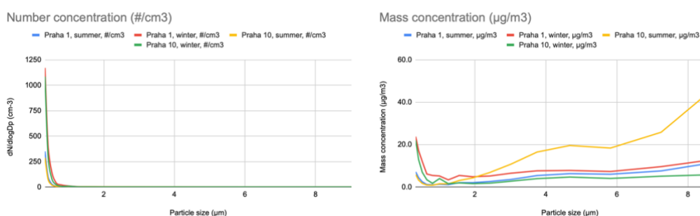
Fig. 12 and 13. Averaged levels of particulate matter outside in both residential areas. Measurements were taken in the summer of 2023 and in the winter of 2024. Fig. 12 (left) represents particle raw counts (#/cm 3 ). Fig. 13 (right) shows mass distributions (µg/m 3 ).
