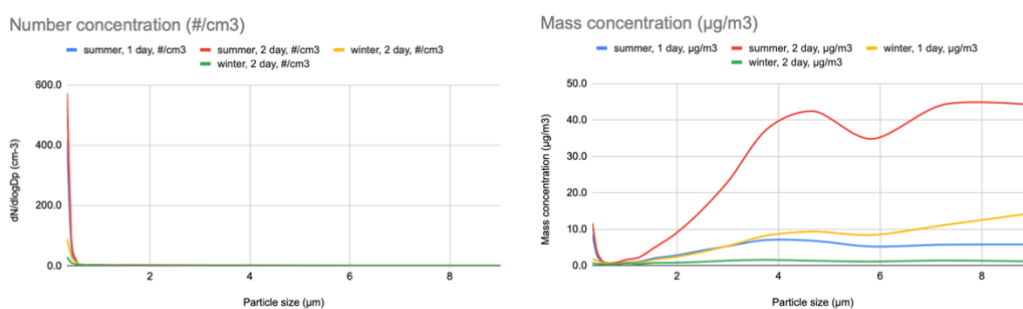
Fig.16 and 17. Averaged levels of particulate matter in the office, in Pruhonice. Measurements were taken in the summer of 2023 and winter 2024. Fig.16 (left) shows particle raw counts ( \#/\text{cm}^3 ). Fig.17 (right) represents mass distributions ( \mu\text{g}/\text{m}^3 ).
