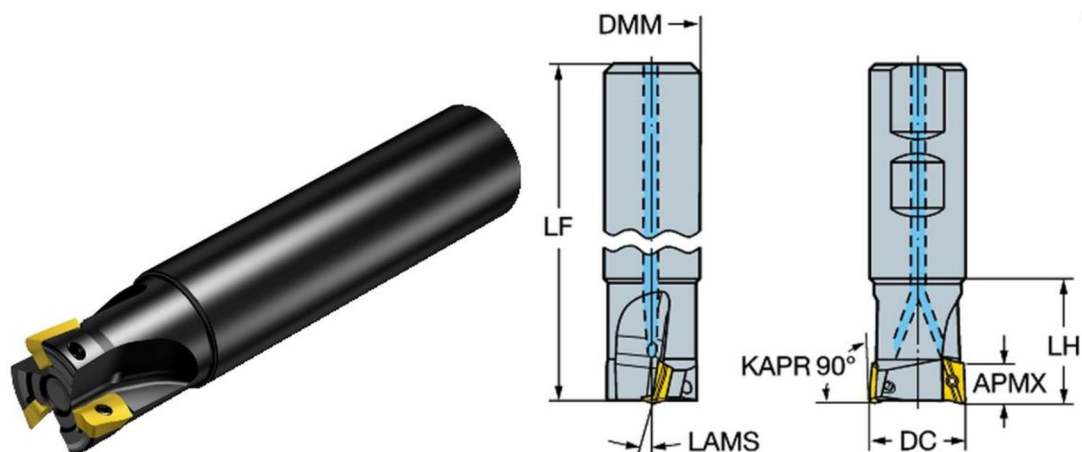
Obr.9 CoroMill 390. [16]
