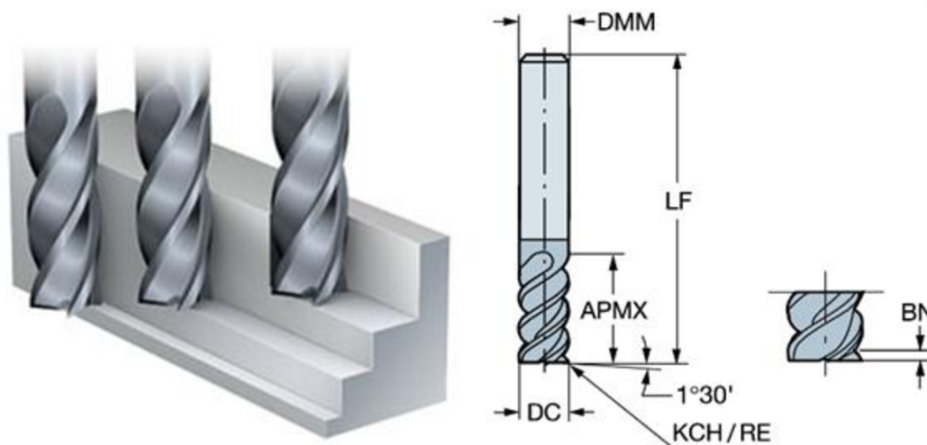
Obr.12 CoroMill Plura 1610. [16]
