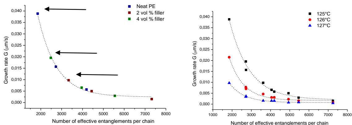
Figure 11: Dependence of the growth rates based on the effective number of entanglements calculated from the crystal growth rates at 125^\circ\text{C} . Shift factors are 1 for neat system, 1.41 for nanocomposite containing 2vol% of silica filler and 1.83 for nanocomposite with 4vol% of fillers, respectively. The arrows show the matrices with in reality the same molecular weight. On the right, plot of the growth rates based on the effective number of entanglements calculated from the crystal growth rates at all temperatures, applying the shift factors from the figure.
