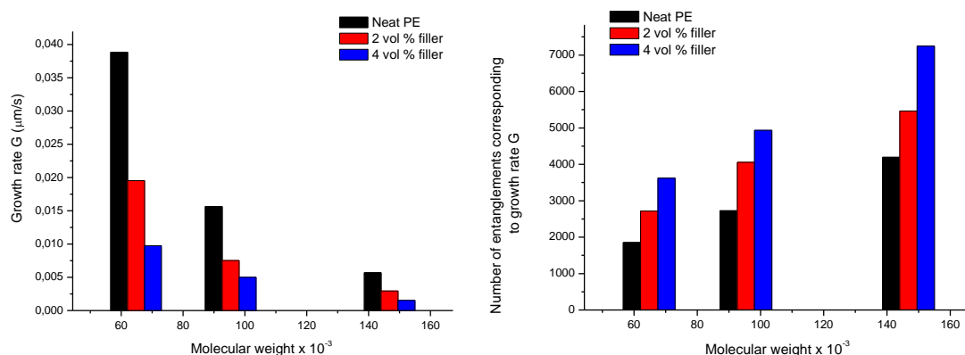
Figure 10: The crystal growth rates at 125^\circ\text{C} . The rate decreases with the increasing of the filler content and with increasing molecular weight of the matrix. On the right, the effective number of entanglements calculated from the crystal growth rates at 125^\circ\text{C} .
