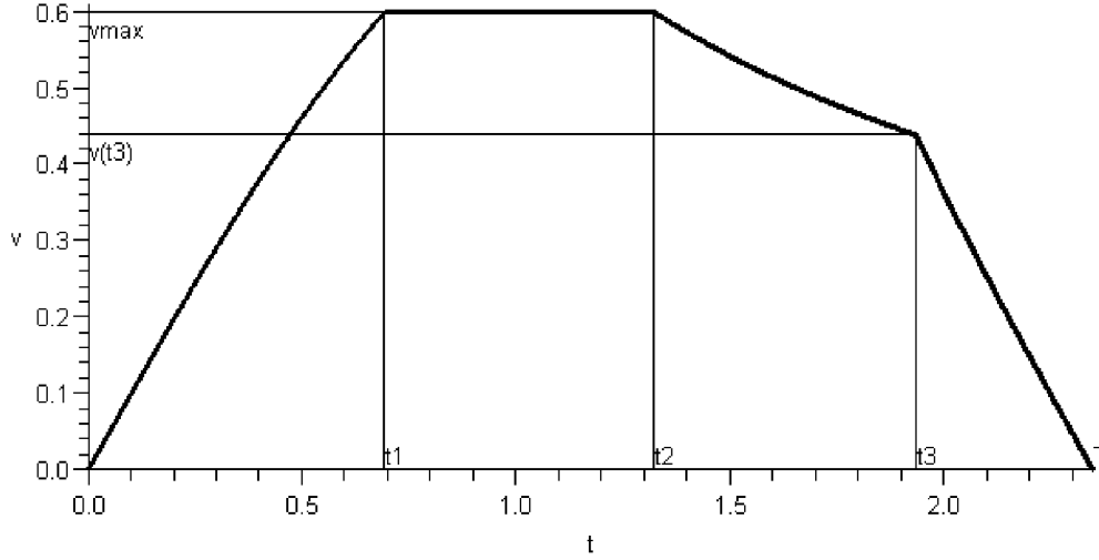
Figure 5.1: A typical speed profile for t_1 < t_2 , parameters \alpha = 1 , \beta = 1 , c = 1 , L = 1 , \gamma = 0.5 , p = 0.7 and r = cv^2
