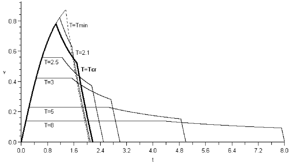
Figure 3.5: Typical speed profiles for parameters \alpha = 1 , \beta = 1 , c = 1 , L = 1 , various values of parameter T and resistance function r = cv^2
