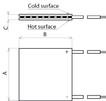
Figure 15 - Thermoelectric Module II.
