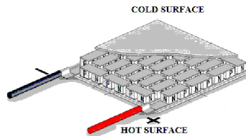
Figure 14 - Thermoelectric module I.
