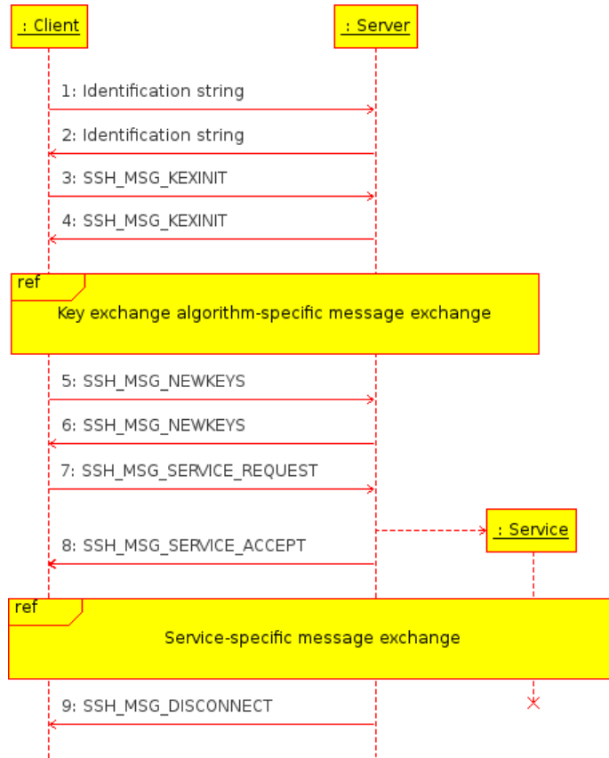
Figure 2.1: Message exchange in SSH transport layer protocol.
