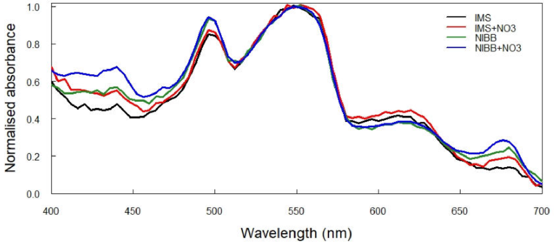
Figure 6.1: Absorption spectra of phycobiliproteins of Trichodesmium erythraeum strains. Absorption is normalised to the average in the vicinity ( \pm 4 nm) of 545 nm. Each curve represents the average of three replicates of a given group.
