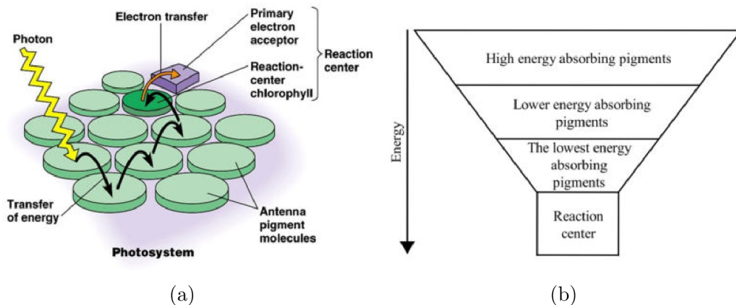
Figure 1.2: The principle of light-harvesting antennas in photosynthetic organisms. (a) Light is absorbed by a pigment either in the antenna pigments or in the reaction center (RC) chlorophyll. Through the antenna system the energy transfer involves migration of electronic excited states which eventually get to the RC where electron transfer takes place, creating an oxidised electron donor and a reduced electron acceptor. (b) The funnel concept of the antenna complexes. The excitation transfers from the pigments absorbing at shorter wavelengths to the ones absorbing at longer wavelengths. (a) Source: Campbell et al. (1996). (b) Source: Blankenship (2021).
