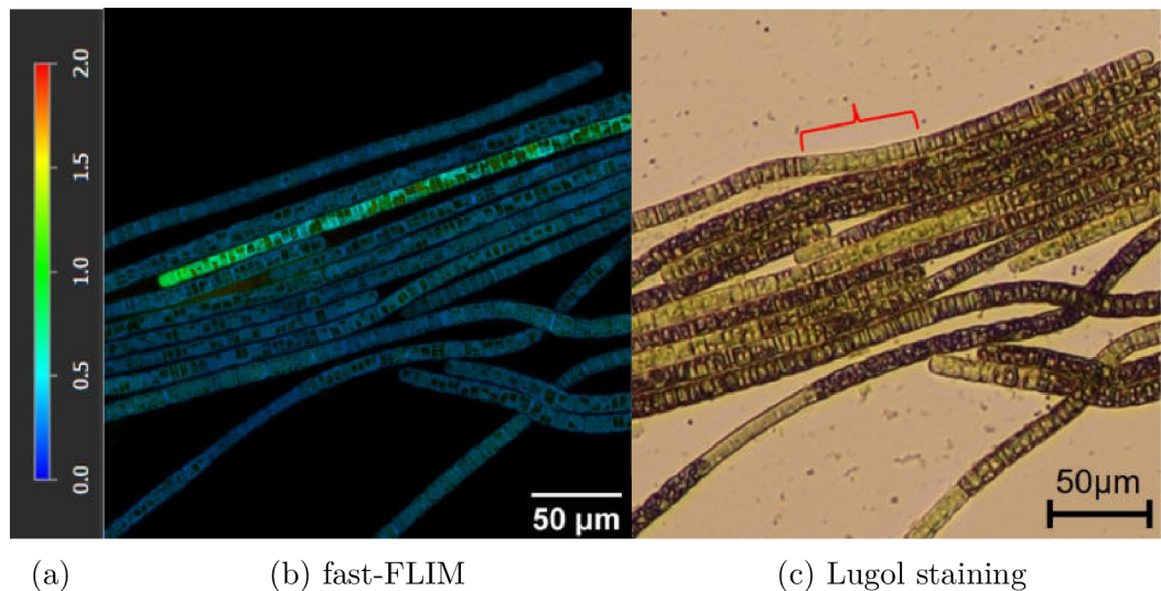
Figure 6.23: Type 7 "unstained". Comparison of pictures of the same sample of N_2 -fixing Trichodesmium IMS101 (b) from FLIM and (c) after staining with Lugol's solution. The red line indicates the unstained segment, which does not show any specific FLIM pattern. (a) The colour scale ranges from 0 to 2 ns.
