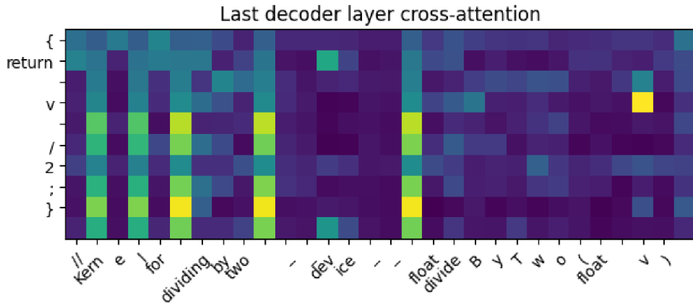
Listing 5.1: Input prompt and model’s generated body for the cross-attention map below.
