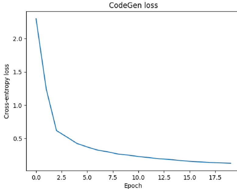
Figure 5.22: CodeGens recorded loss value throughout the training process. The maximum value of 2.3, Minimum in the last epoch of 0.127 average per epoch.
