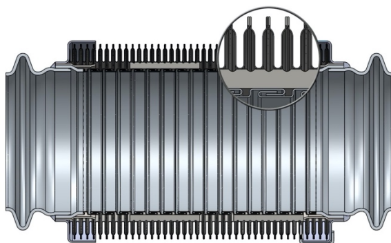
Obr. 8: Gastight hose – GTH (wesfalia-mh.com, 2020)
