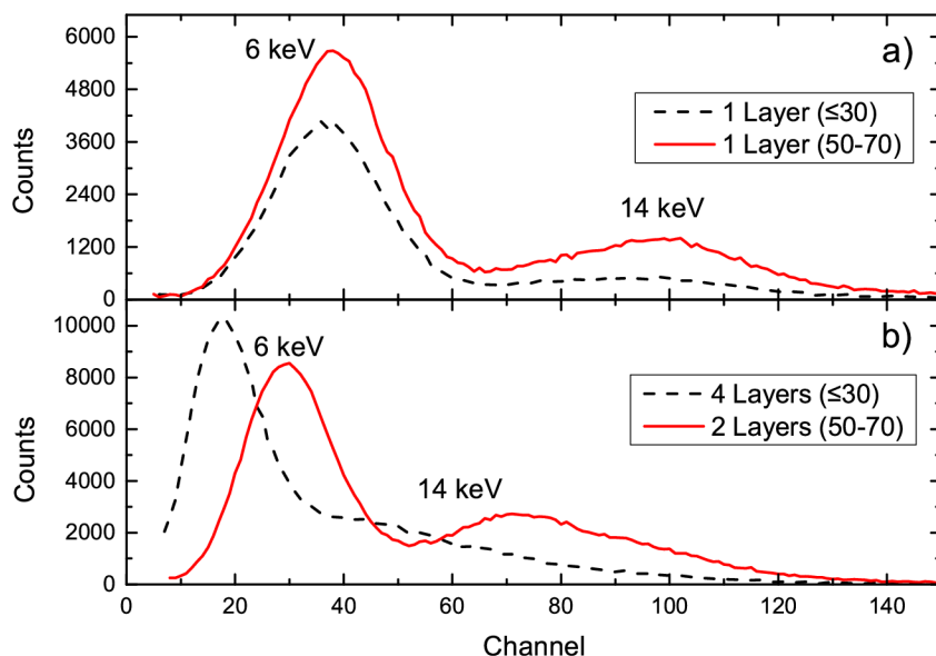
Fig. 4. Amplitude spectra of (a) one \le 30\ \mu\text{m} layer and one 50–70 \mu\text{m} layer, (b) four \le 30\ \mu\text{m} layers and two 50–70 layers.
