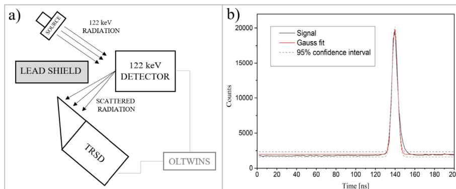
Fig. 4. (a) The experimental setup for measurement of time resolution of the TRSD. (b) Measured coincidence time resolution of the TRSD.
