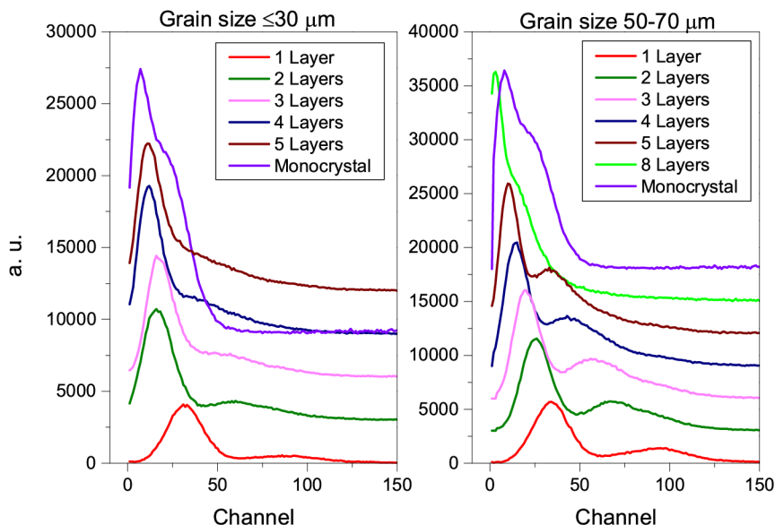
Fig. 5. Amplitude spectra for 1 to 5 layers for the granularity \le 30\ \mu\text{m} and 1 to 8 layers for the granularity 50–70 \mu\text{m} .
