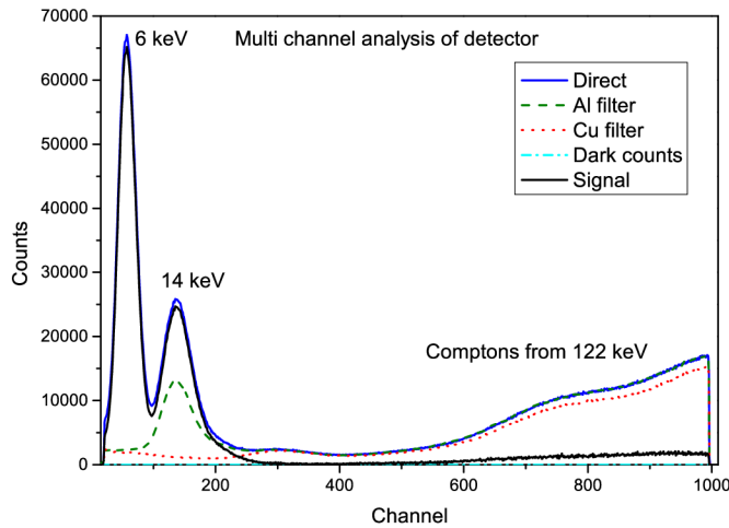
Fig. 1. Instrumental spectra of ^{57}\text{Co} , blue—direct beam, green—Al filtered beam, red—Cu filtered, cyan—dark counts and background, black—signal. (For interpretation of the references to colour in this figure legend, the reader is referred to the web version of this article.)
