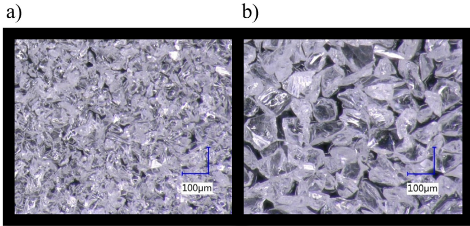
Fig. 1. YAP:Ce powder on adhesive tape with grain size of (a) \leq 30 \mu\text{m} and (b) 50\text{--}70 \mu\text{m} .
