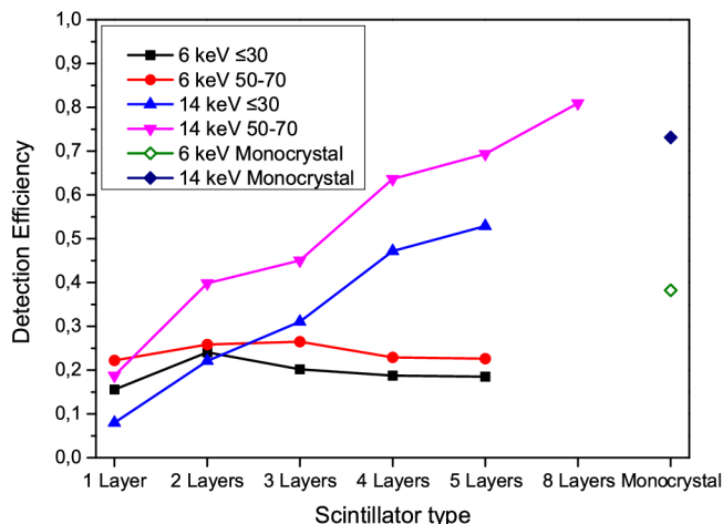
Fig. 6. Detection efficiencies for 1 to 8 layers for the granularities \leq 30 \mu\text{m} , 50\text{--}70 \mu\text{m} and the monocrystal.
