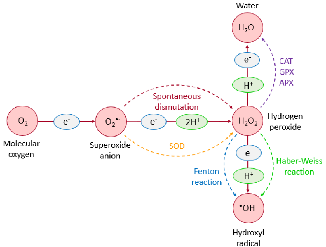
Figure 2: Electron transport showing sequential formation of O_2^{\bullet-} , hydrogen peroxide ( H_2O_2 ) and HO^{\bullet} formation from molecular oxygen.
