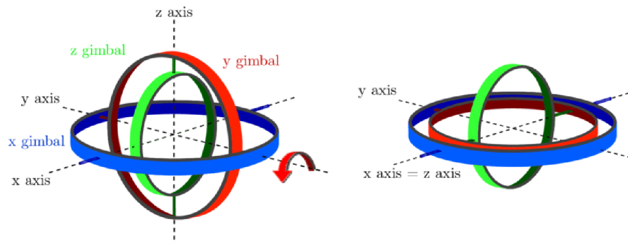
Obr. 4: Gimbal-lock [11]
