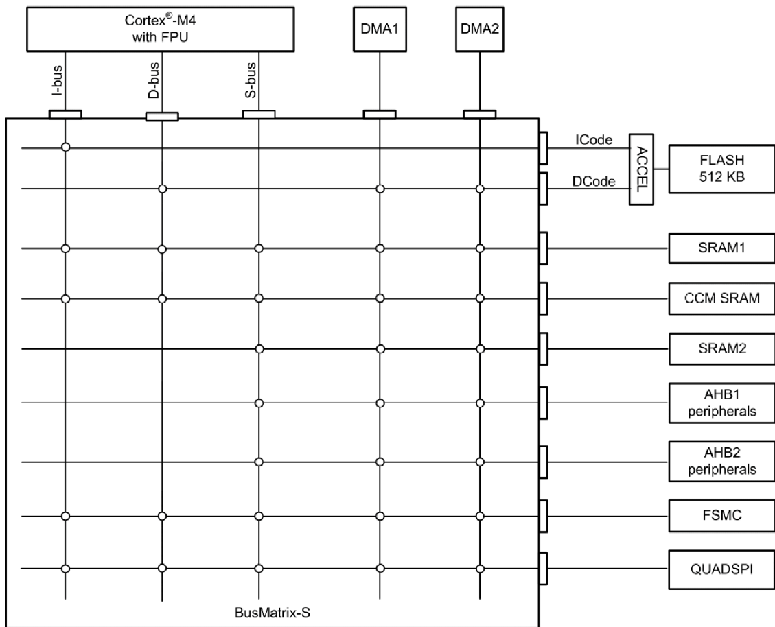
Obr. 27: BusMatrix [41]
