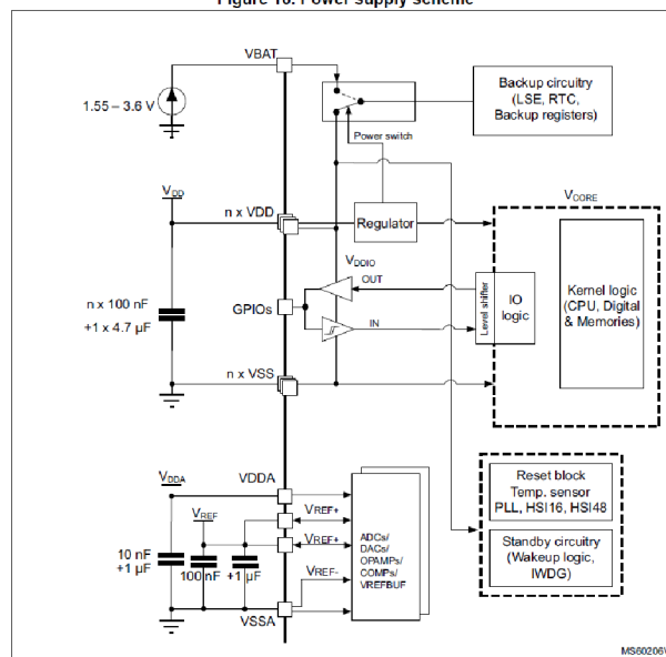
Figure 16. Power supply scheme
