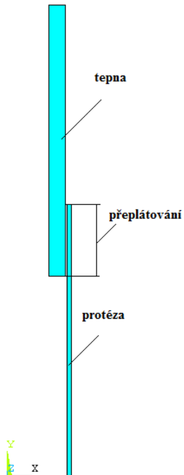
Obr. 6.1: Model geometrie
