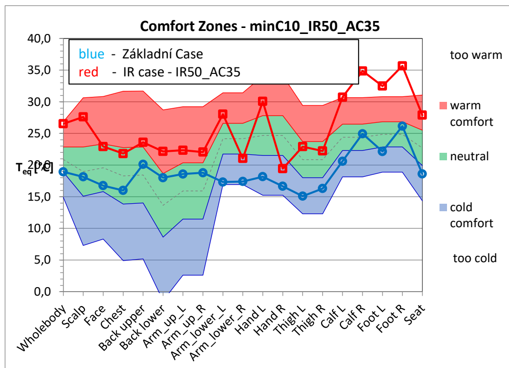
Graf 3.35.50: Case T_{amb} = -10\text{ °C} T_{IR} = 50\text{ °C} T_{AC} = 35\text{ °C}
