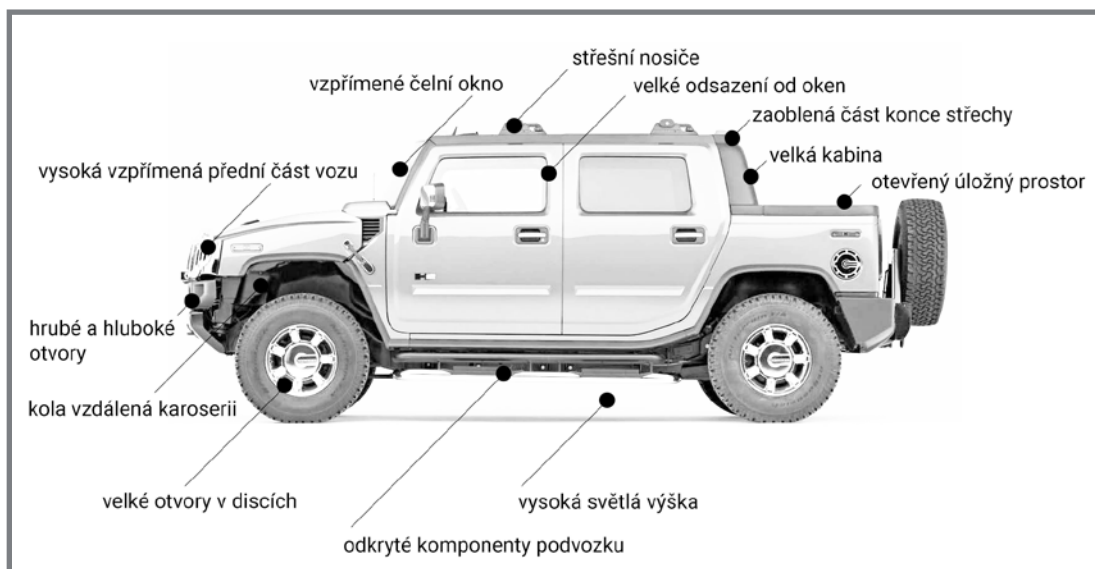
Obr. 2-14 Hummer H2T [3]
