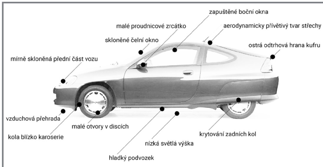
Obr. 2-13 Honda Insight [3]
