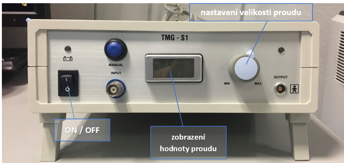
Obr. 4.3: Potenciostat
