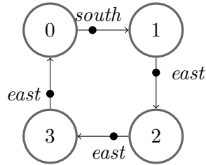
(b) FSC synthesized from a design space restricted using the Simple circle predicate
