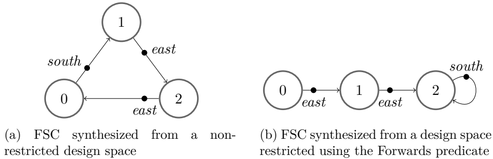
Figure 6.4: FSC controllers with memory size 3 synthesized for the Grid Avoid benchmark
