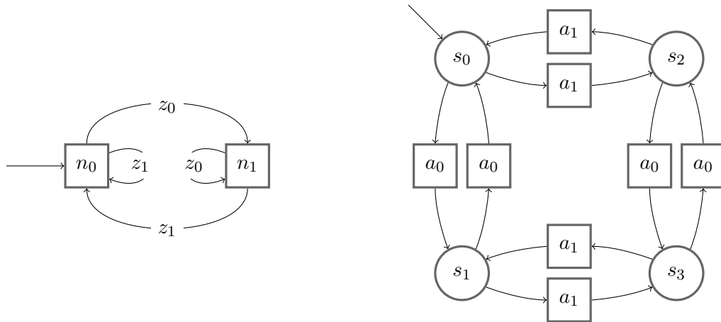
Figure 3.2: Finite-state controller F (left), POMDP \mathcal{M} (right)
