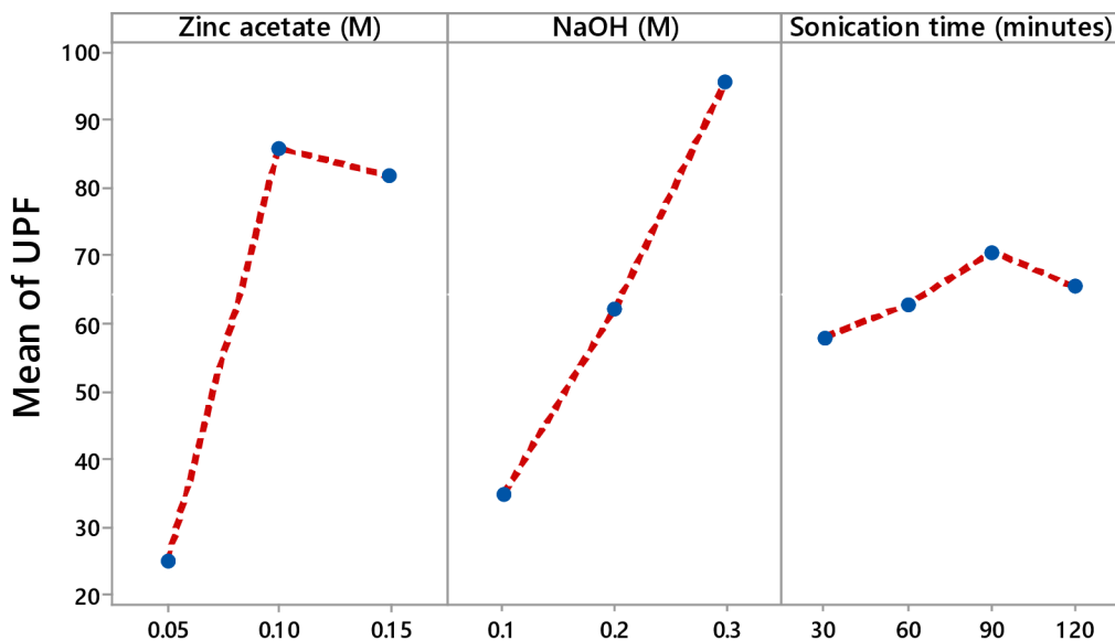
Figure 42. Main effects plots for UPF.
