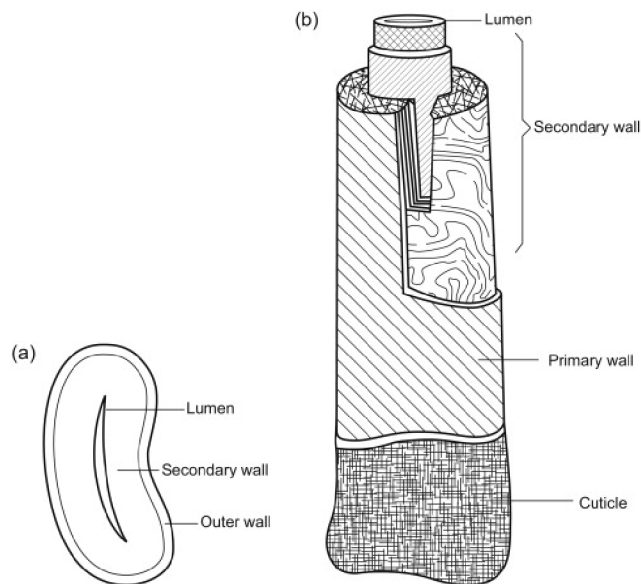
Figure 4. Structure of cotton fiber. (a) cross-section of fiber, (b) vertical section of fiber [64].
