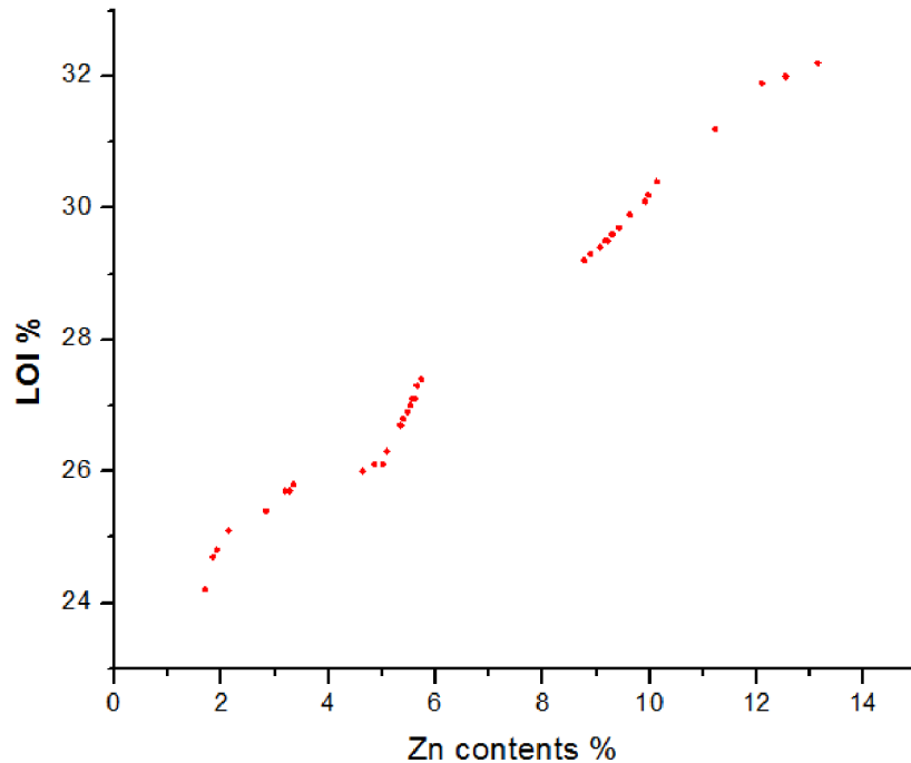
Figure 36. Graphical representation of LOI values vs Zn contents %.
