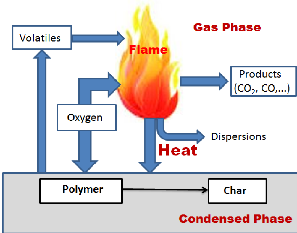
Figure 9. Polymer combustion cycle[124].
