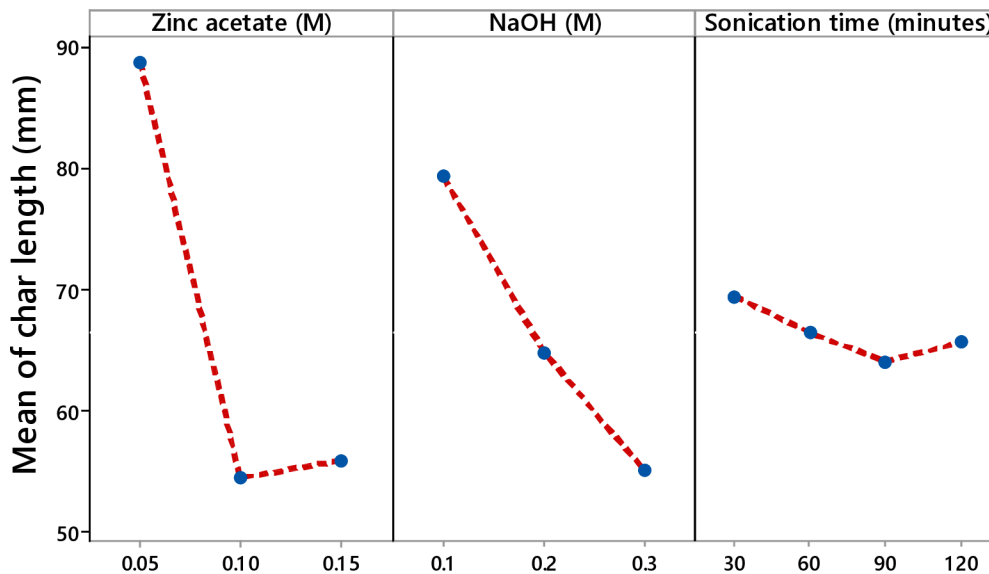
Figure 35. Main effects plots for char length (mm).
