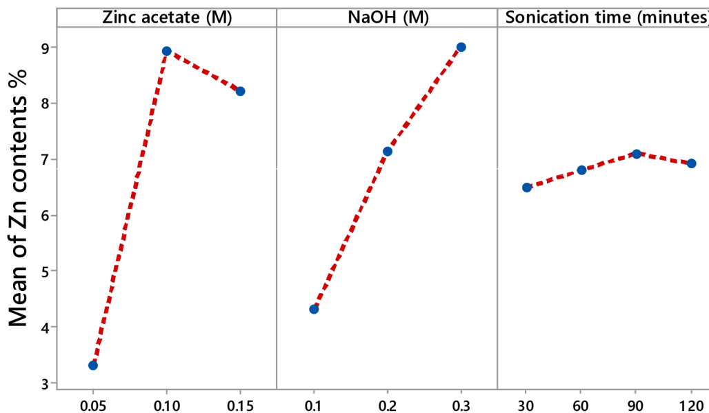
Figure 26. Main effects plots for Zn contents %.
