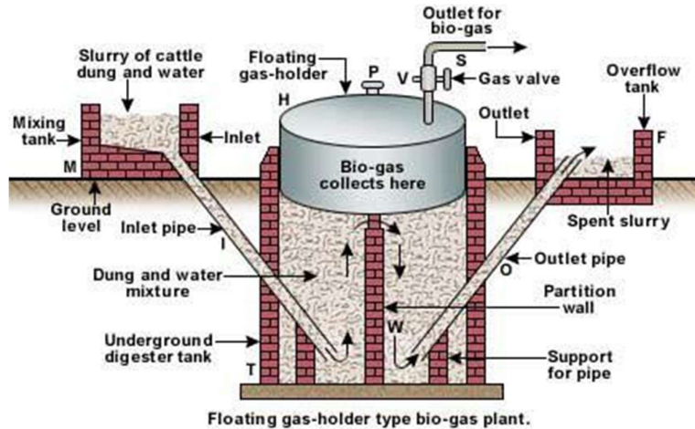
Figure (5): Floating drum biogas digester adapted from Biogas Potential in Pakistan by Saleh A., (2012)
