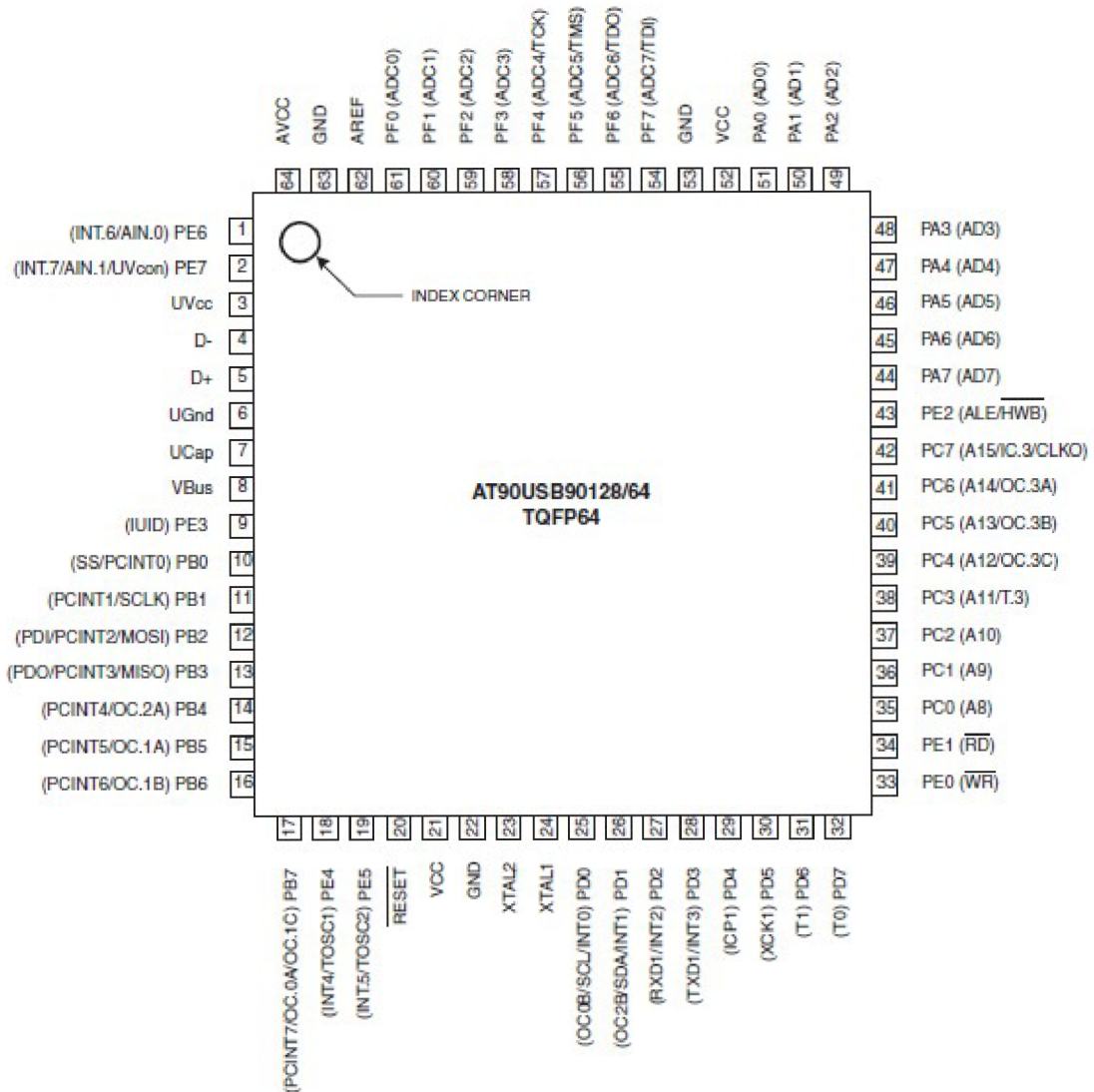
Obr. 2.1: Zapojenie AT90USB1287 [3]
