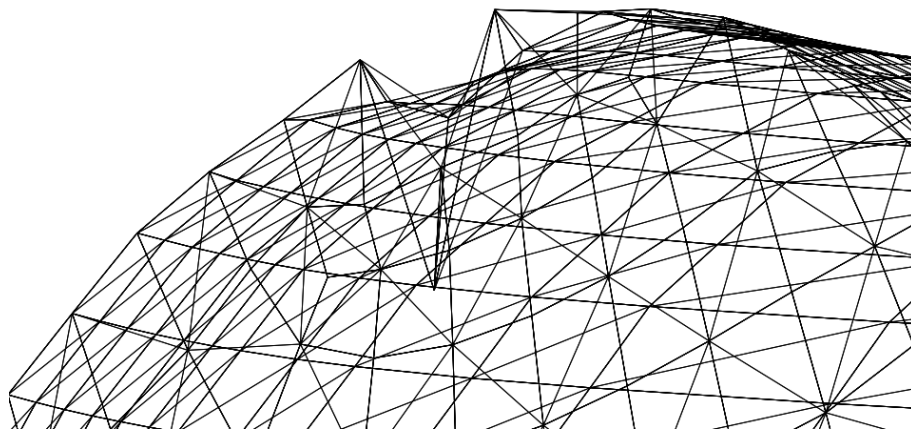
Obr. 2.7: Detail singularity
