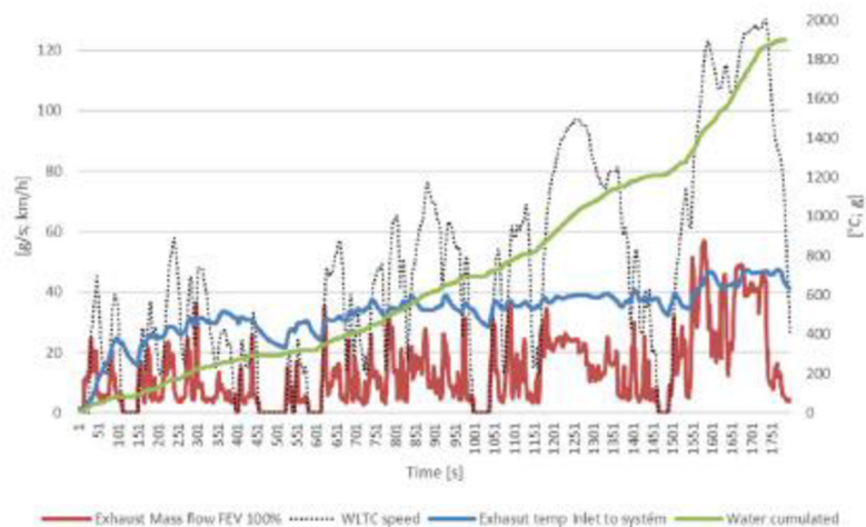
Figure 6. Data from the vehicle test.
