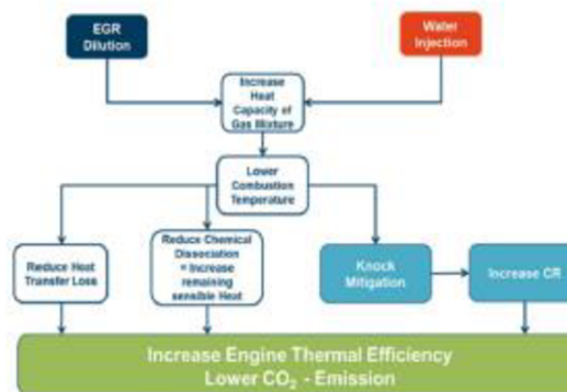
Figure 2. Summarizes the respective effects of EGR and Water Injection.
