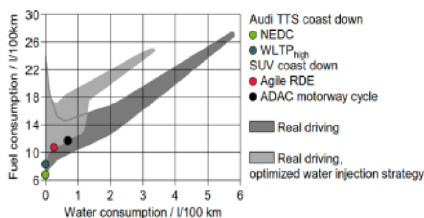
Figure 5. Water Consumption for Various Test Conditions [12].
