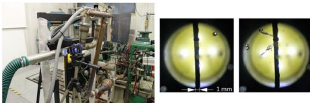
Figure 12. Condensate droplets size measuring.
