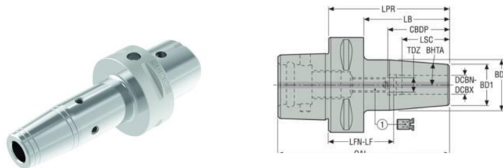
Obr. 35 Upínač C6-391.5603-06080 [16].
