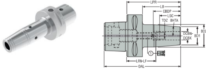
Obr. 28 Upínač C6-391.5603-10080 [16].
