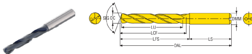
Obr. 37 Vrták SD_DRILL_3.0MM_5XD_A [16].
