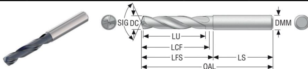
Obr. 34 Vrták SD_DRILL_8.9MM_3XD.
