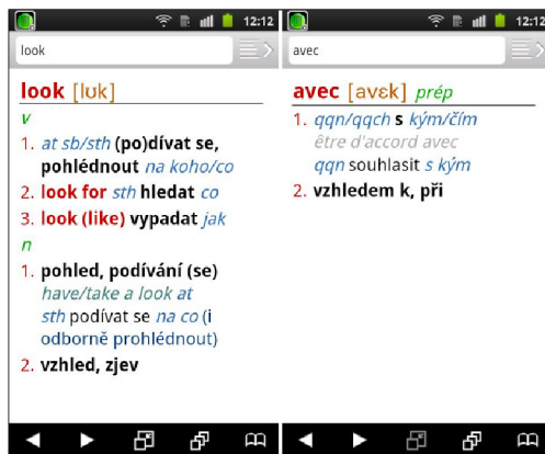
Obr. 3.3: HandyLex 4 Czech
