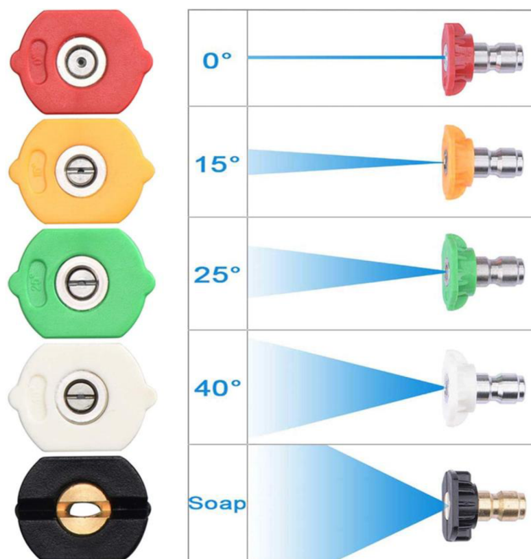
obr. 6-5 Trysky [32]
