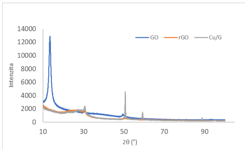
Obr. 14: XRD spektra GO, rGO a Cu/G
