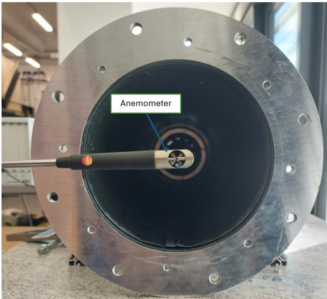
Figure 7 Anemometer Positioning
