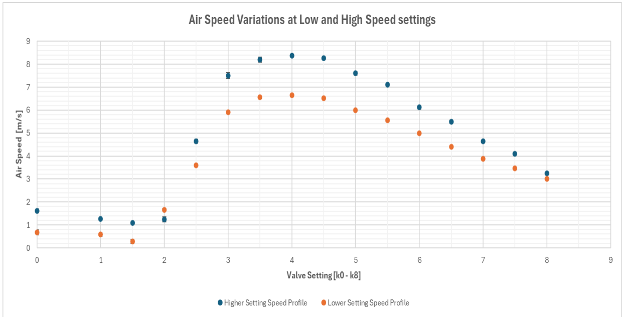
Figure 10 Air Speed Variations at Low and High-Speed Settings
