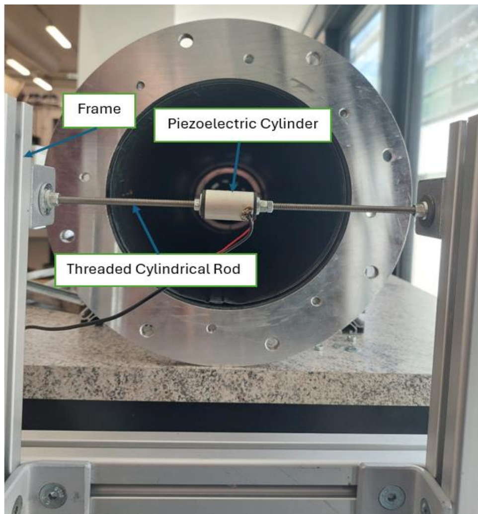
Figure 6 Cylinder Configuration
