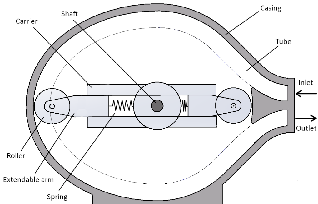
Figure 22 – Schematic of elliptic peristaltic pump
