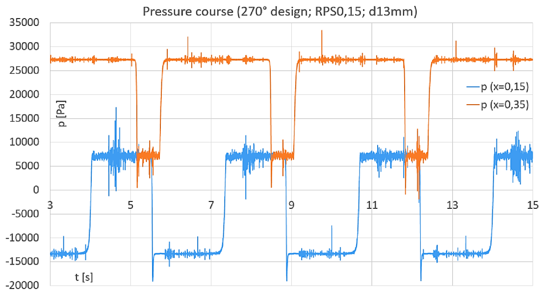
Figure 38 – pressure course (270° design; RPS = 0,15 1/s; d_{tube} = 13\text{ mm} )
