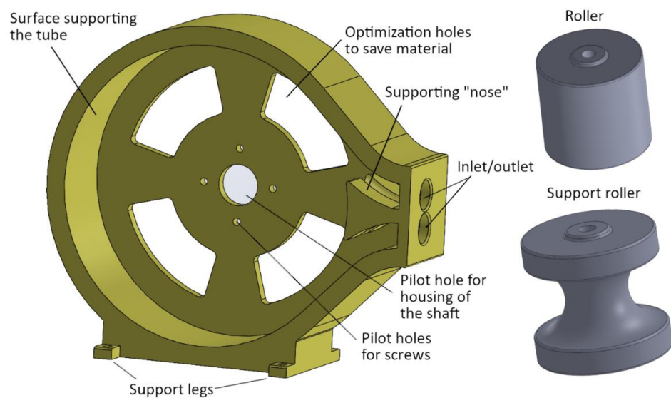
Figure 20 –Casing (left), support roller (bottom right), roller (top right)
