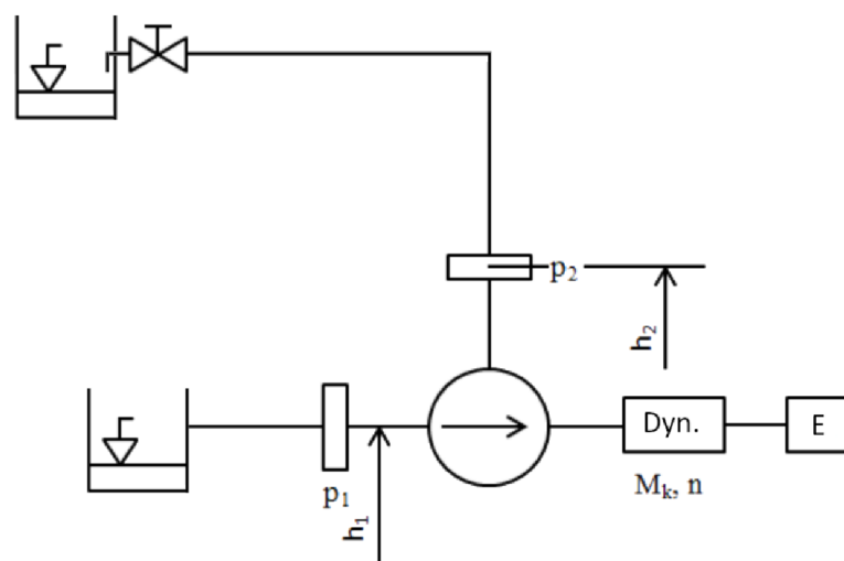
Figure 40 – Scheme of the experimental circuit
