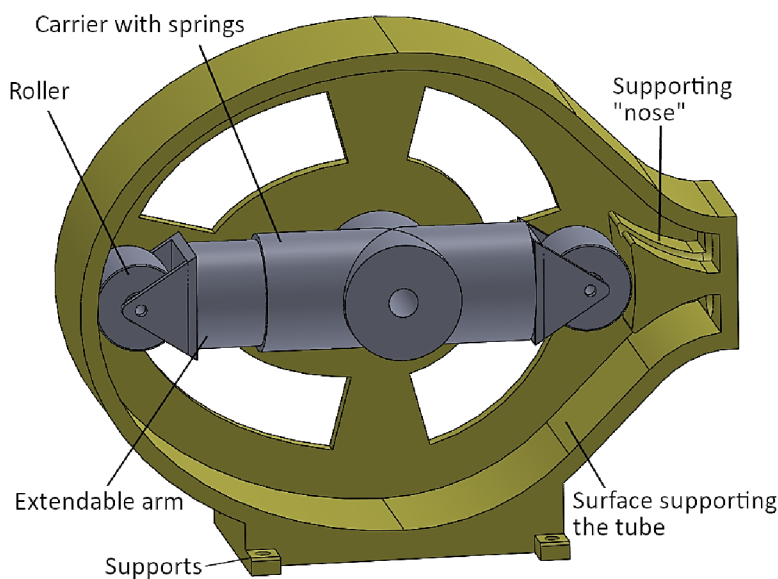
Figure 23 – First design of elliptic peristaltic pump
