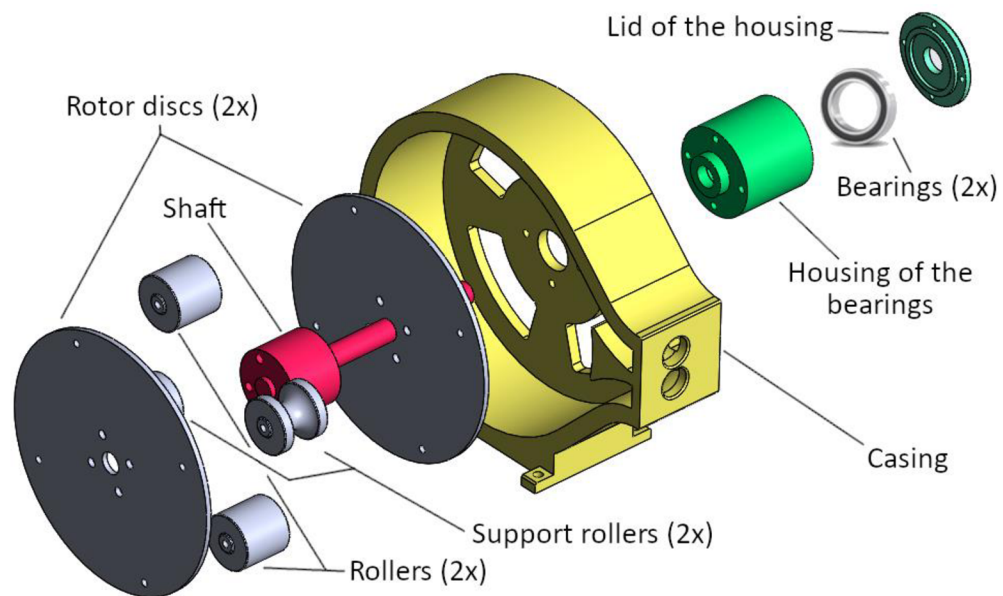
Figure 19 – Dismantled design of peristaltic pump
