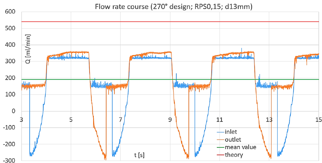
Figure 36 – Flow rate course (270° design; RPS = 0,15 1/s; d_{tube} = 13 mm )
