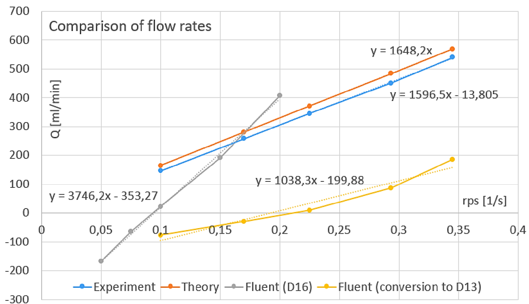
Figure 45 – Final comparison of flow rates
