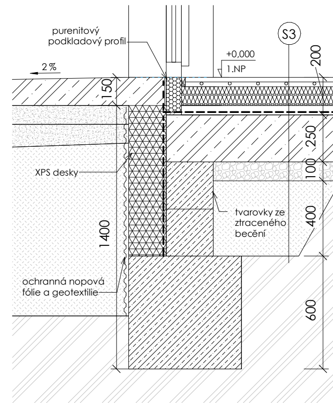
Detail 1:20
