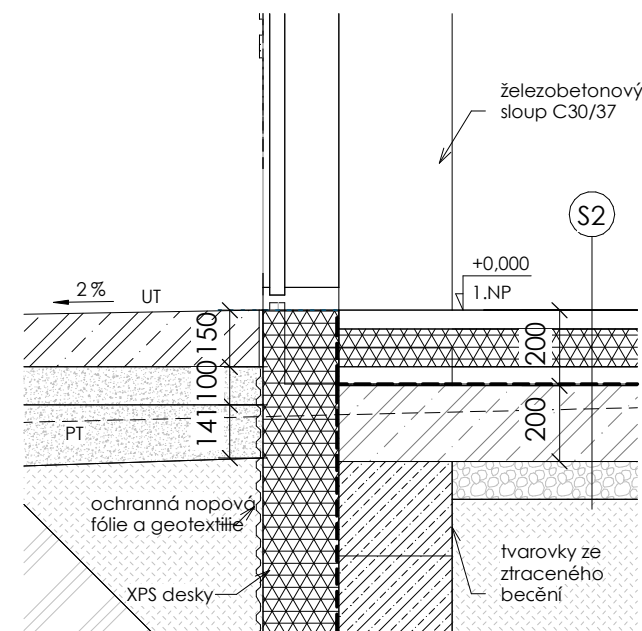
Detail 1:20
