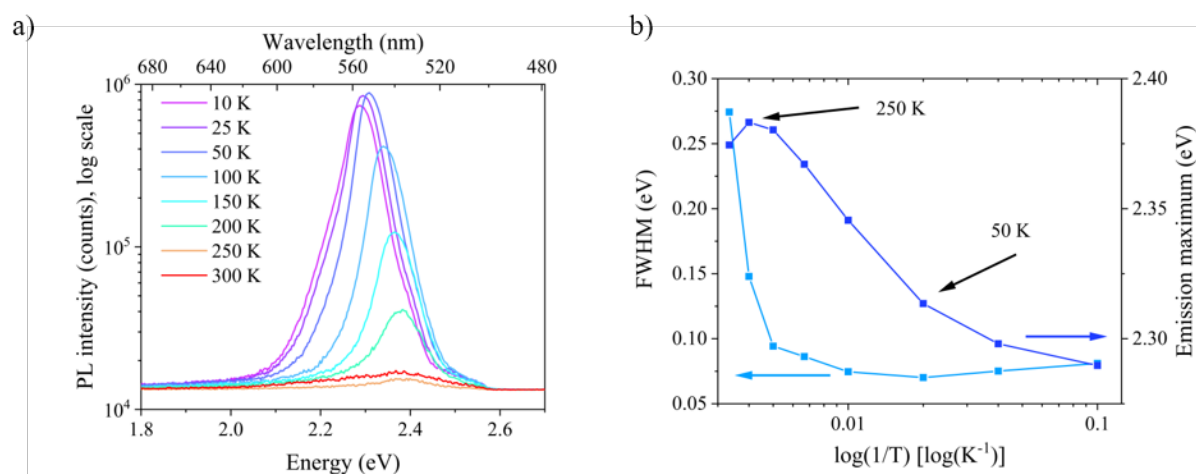
Figure 56: a) PL spectra of PNA-M-PNP film detected at different temperature, b) dependency of FWHM and emission maxima on temperature
