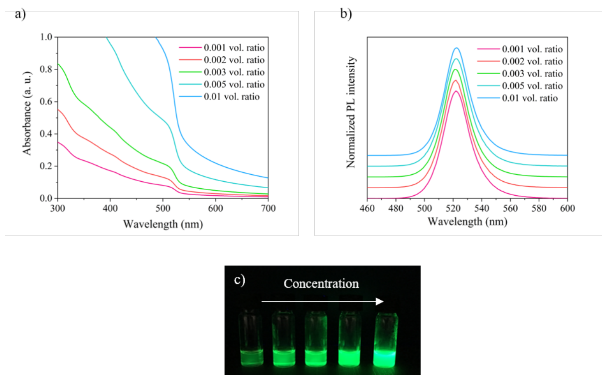
Figure 14: Optical properties of colloidal solutions prepared by precipitating precursor solution in toluene in different volume ratios, a) absorption spectra, b) emission spectra and c) image of corresponding samples under UV irradiation (366 nm)
