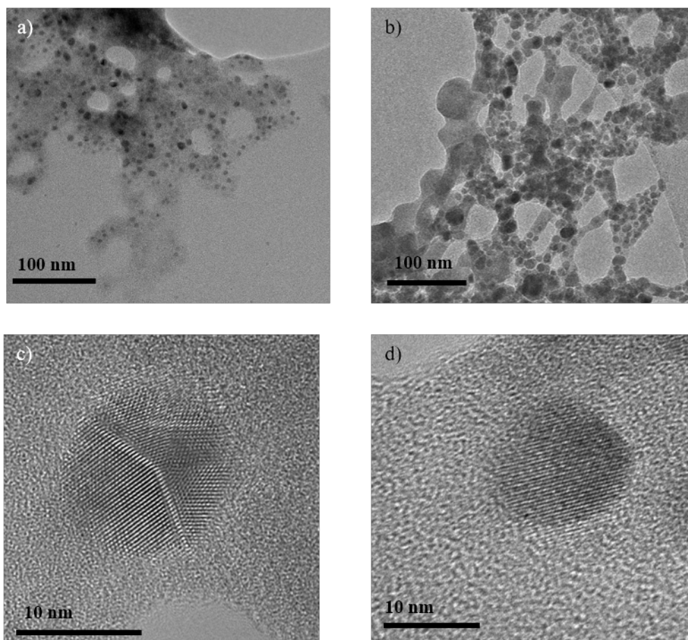
Figure 13: TEM images of PNP, a) aggregates formed in the crude sample and b) in three times washed sample, c) individual nanoparticle from the crude sample and d) from three times washed sample
