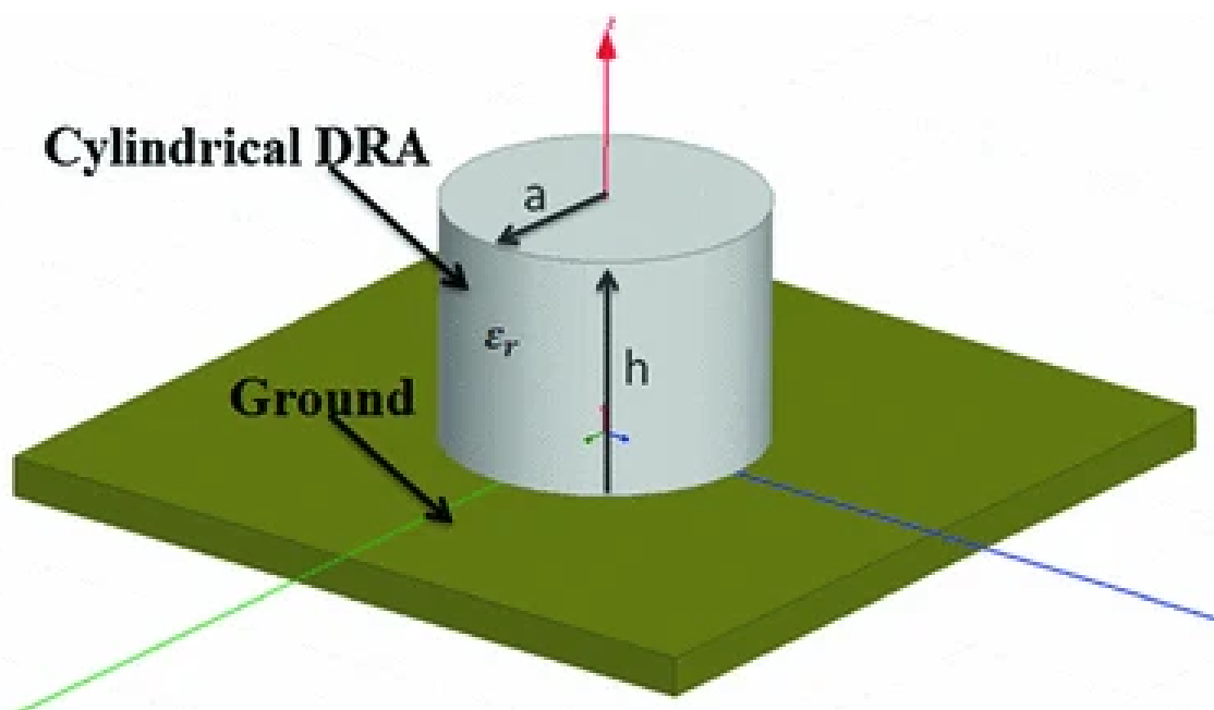
Fig. 2.1: Parameters of the cylindrical DRA[5]
