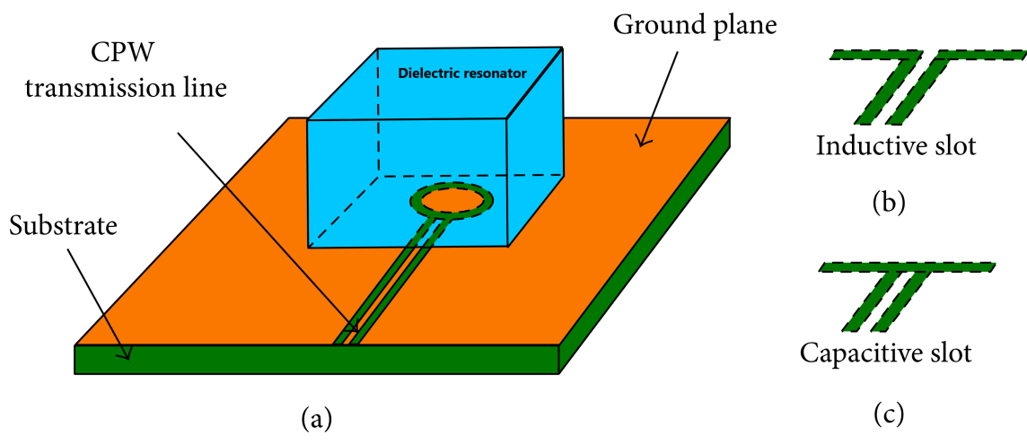
Fig. 1.5: Coplanar-waveguide coupling[4]
