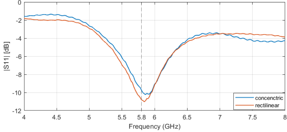
Fig. 5.11: Measured reflection coefficient for concentric and rectilinear infill ( \epsilon_r = 7.9 )
