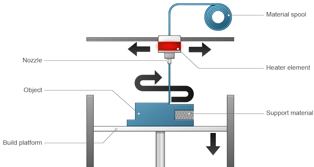
Fig. 3.2: Assembly of material extrusion 3D printer[8]
