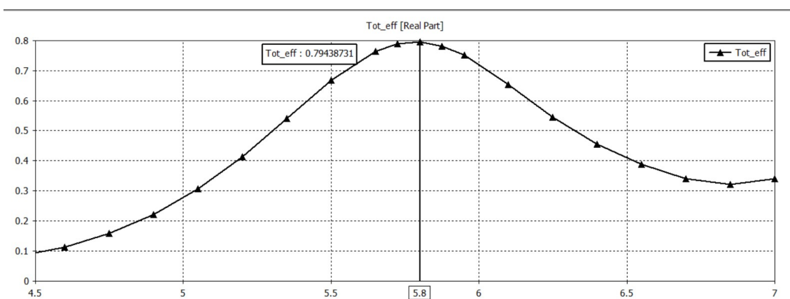
Fig. 4.16: Total efficiency for aperture coupled model
