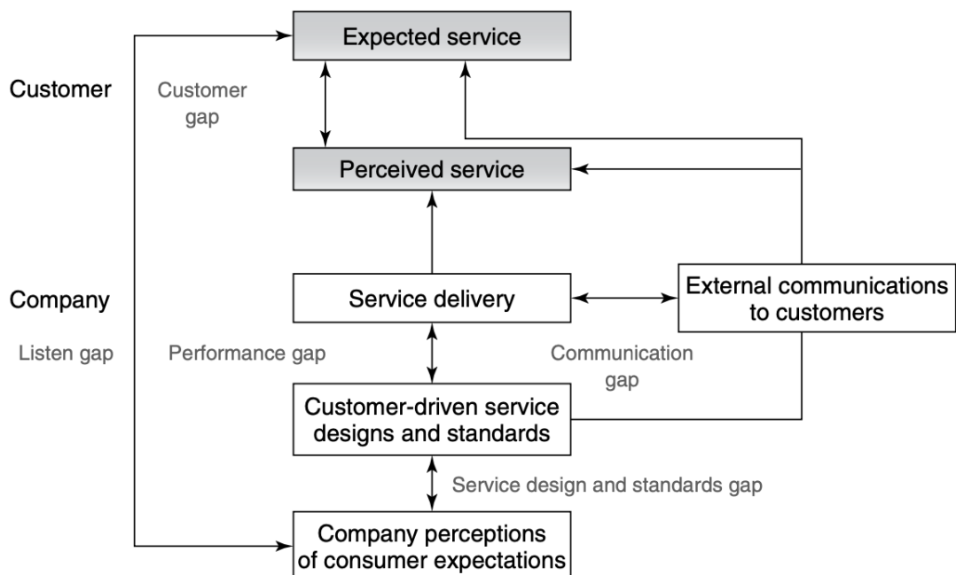
Figure 3 GAP model
