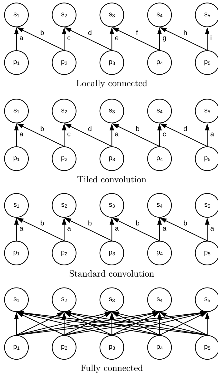
Figure 3.9: Comparison of convolutional layers.
