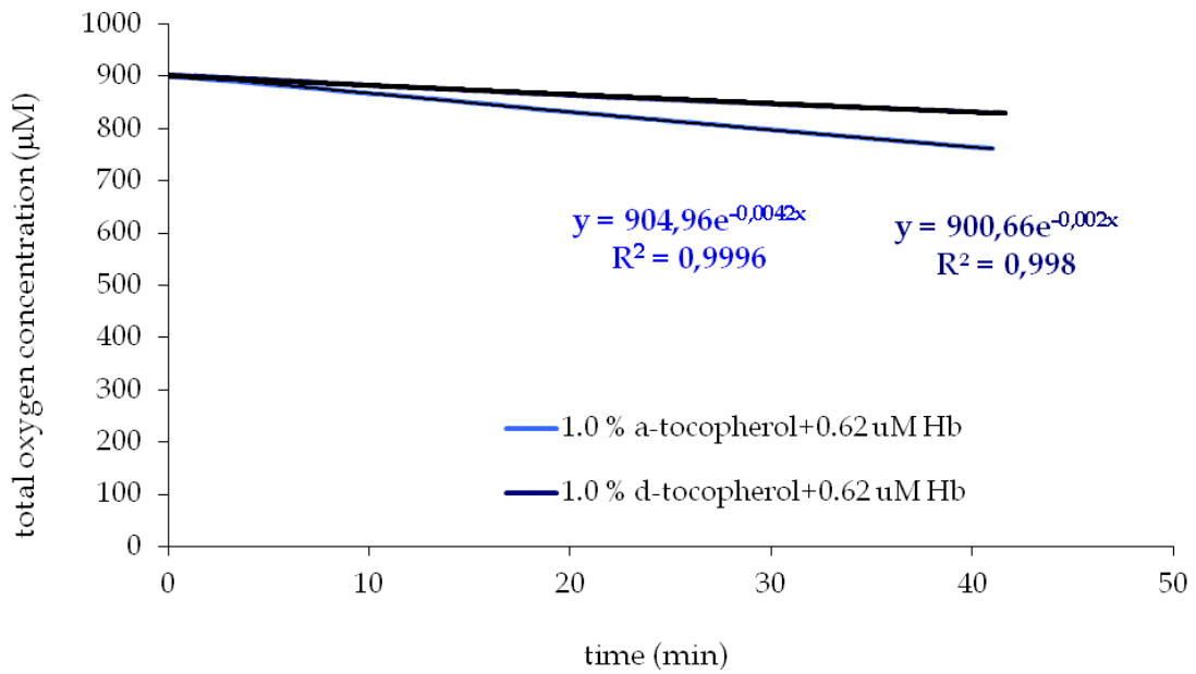
Figure 54: Effect of 1.0 % of \alpha - and \delta -tocopherols on lipid oxidation induced by metHb (0.62 \mu M). The exponential trendlines and their equations are shown
