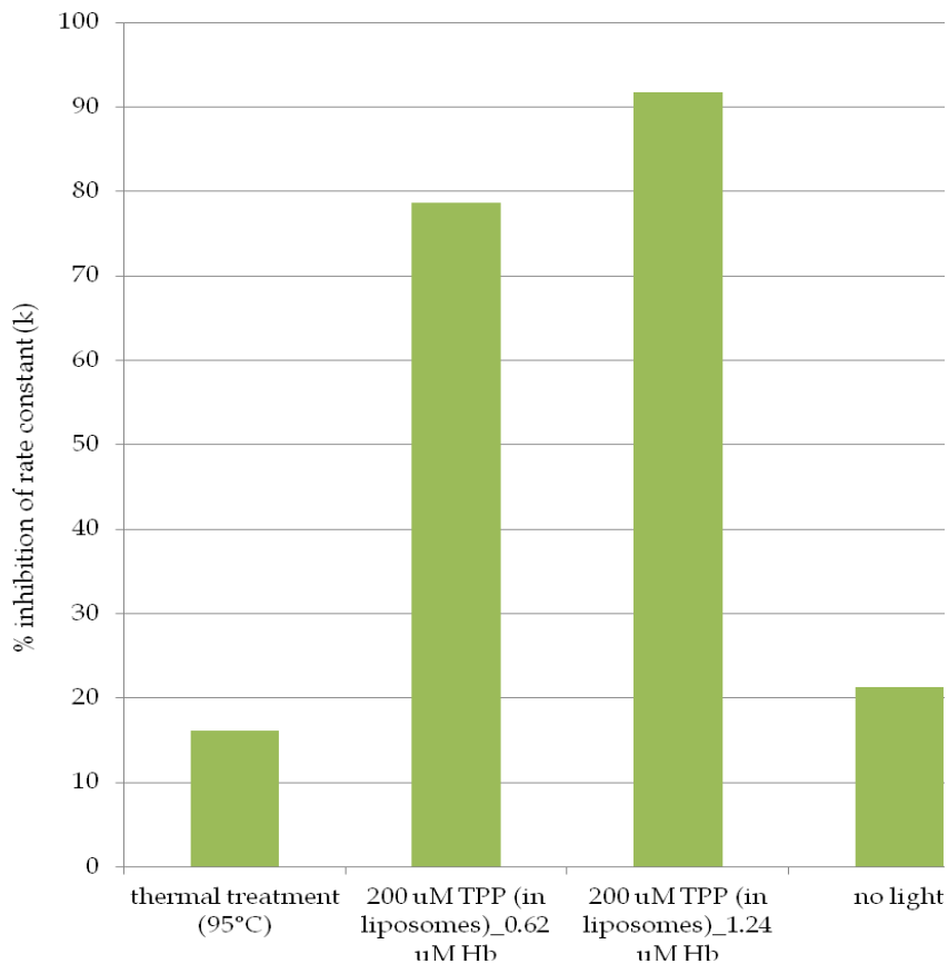
Figure 63: Effect of thermal treatment, TPP and absence of light on the prooxidant activity of metHb (0.62 µM)
