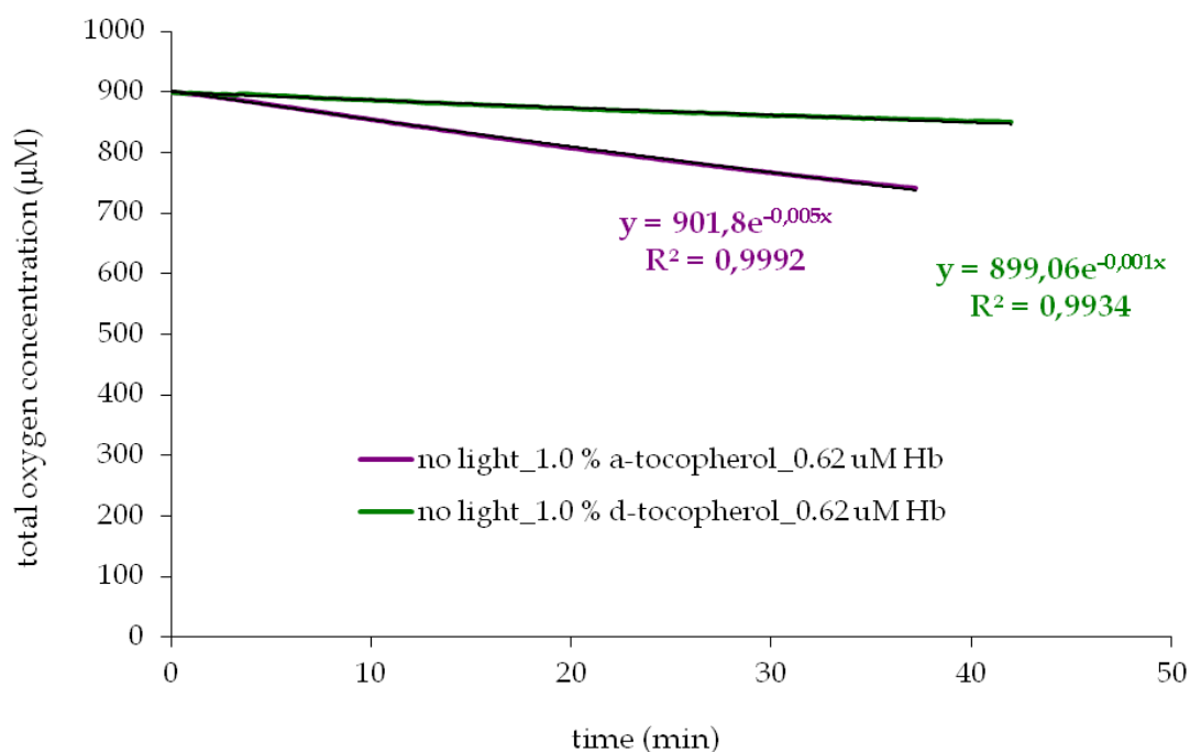
Figure 58: Effect of tocopherols on lipid oxidation of liposomes containing 1.0 % of \alpha - and \delta -tocopherol. The oxidation was induced by metHb (0.62 \mu M). The reaction was run in the absence of light. The exponential trendlines and their equations are shown
