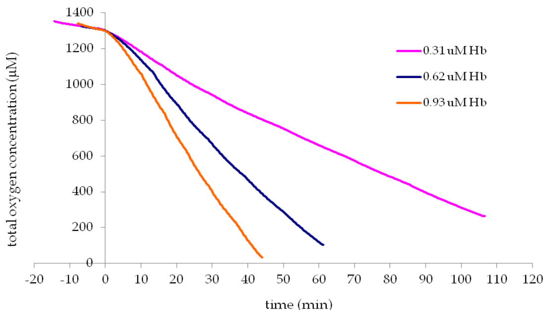
Figure 34: Oxygen consumption of a 1.5% liposome solution; oxidation was catalyzed by metHb added in three different amounts (giving 0.31, 0.62 and 0.93 \mu\text{M} concentration in the reaction cell)
