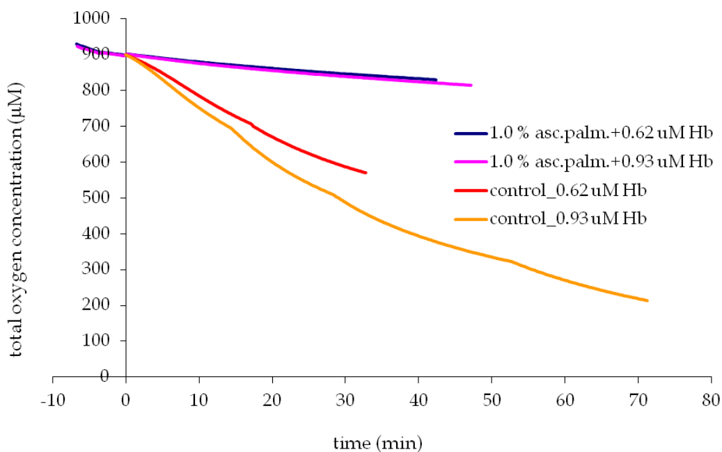
Figure 61: Effect of 1.0 % of ascorbyl palmitate on lipid oxidation induced by metHb (0.62 and 0.93 \mu\text{M} ). The red and orange curves represent control experiments (without AOX)
