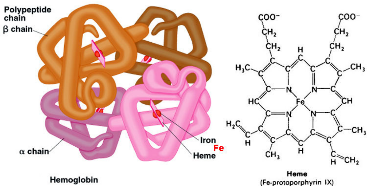
Figure 6: Model of hemoglobin and the structure of heme-group [47]
