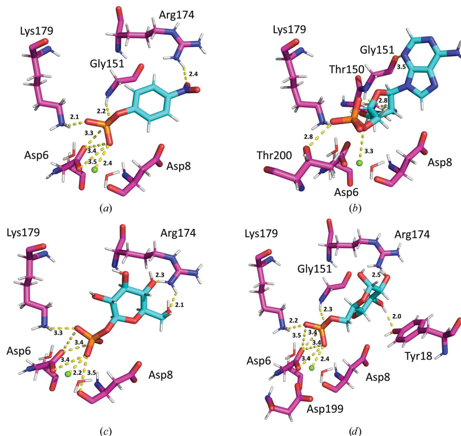
Figure 4 Predicted substrates docked in the active site of Tt82: (a) para -nitrophenyl phosphate (pNPP), (b) adenosine monophosphate (AMP), (c) D-glucose 1-phosphate and (d) D-glucose 6-phosphate. C atoms of Tt82 residues are shown in magenta and C atoms of ligands are in cyan. O atoms are depicted in red, N atoms in blue and P atoms in orange. The magnesium ion in Tt82 is shown as a green sphere. Distances between hydrogen-bond donors and acceptors are shown in Å.
