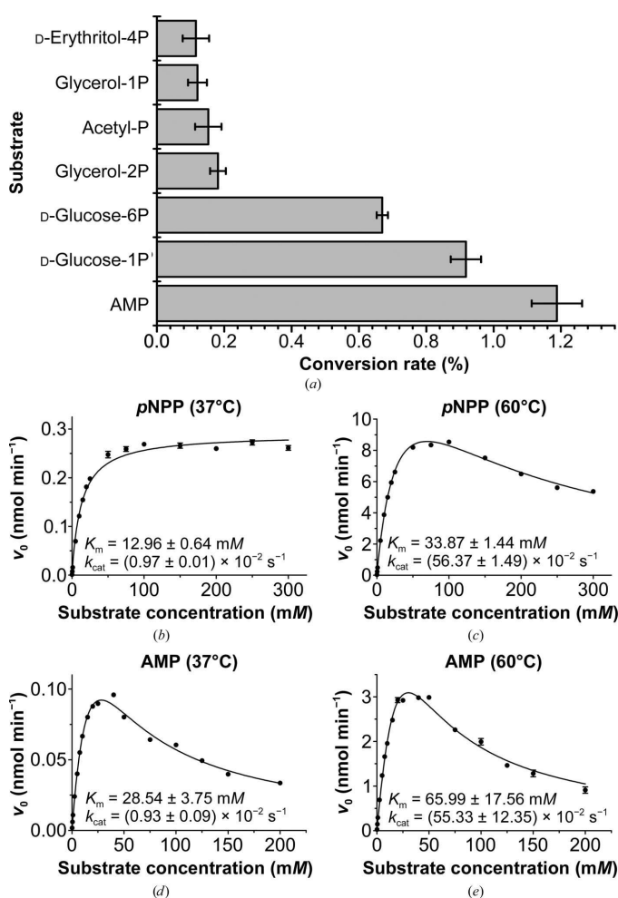
Figure 5 Phosphatase activity of Tt82. (a) Conversion rates of selected compounds assayed by the EnzChek Phosphate Assay Kit. (b)–(e) Steady-state kinetics of para -nitrophenyl phosphate ( p NPP) and AMP at two different temperatures (37 and 60°C). At higher substrate concentrations inhibition by substrate was observed (see the text for details).
