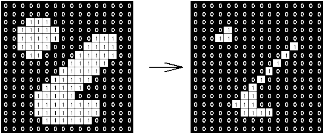
Figure 19: Effect of erosion using a 3×3 square structuring element. [30]
