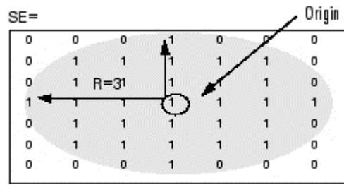
Figure 18: Multidimensional structure element ‘disk’, with radius R=3^1 . Ones represent pixels included in the morphological computation, and zeros are excluded. Origin is the center pixel of the structuring element being processed. [30]
