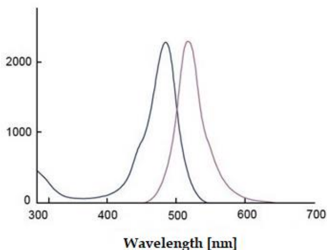
Figure 14: Calcein AM fluorescent spectra. [23]
