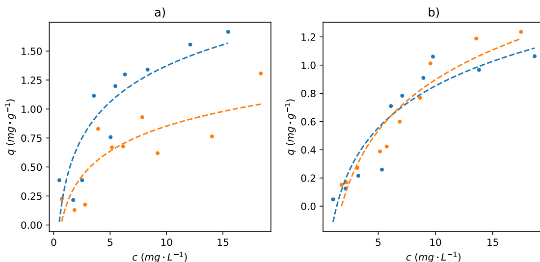
Figure 4.2: Measured data points of adsorption isotherms for Hg: a) fresh water, b) sea water; smaller PET fraction ( < 0,63 \mu\text{m} ) - blue, bigger PET fraction ( 0,63 \mu\text{m} - 1 \text{mm} ) - orange.
