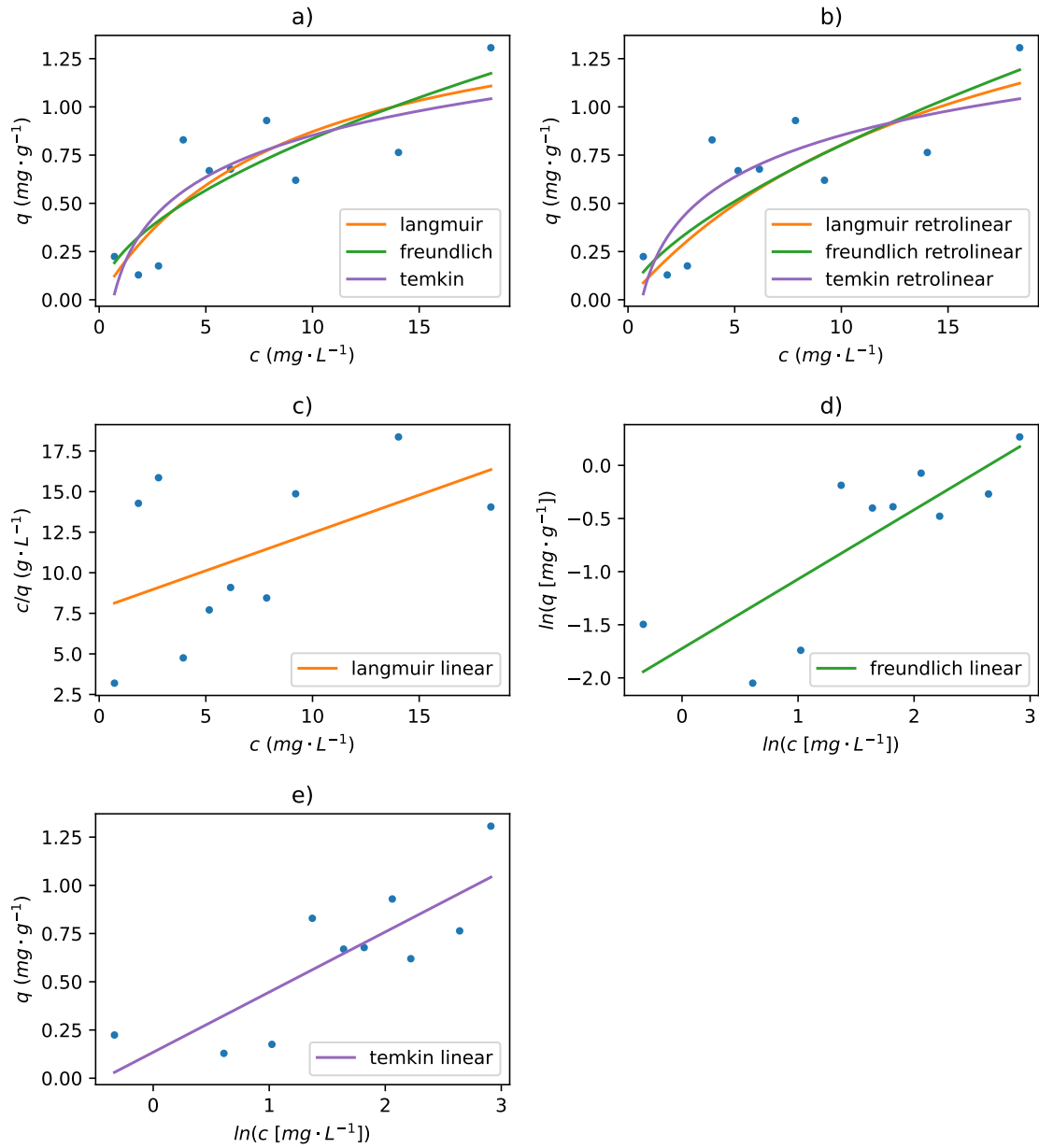
Figure A.6: Adsorption isotherms and their linearised forms for adsorption of Hg on bigger fraction PET (0,63 \mu\text{m} – 1 mm) in freshwater: a) adsorption isotherms constructed from non-linear fitting; b) adsorption isotherms constructed from linear fitting; c) Langmuir linear regression; d) Freundlich linear regression; e) Temkin linear regression.
