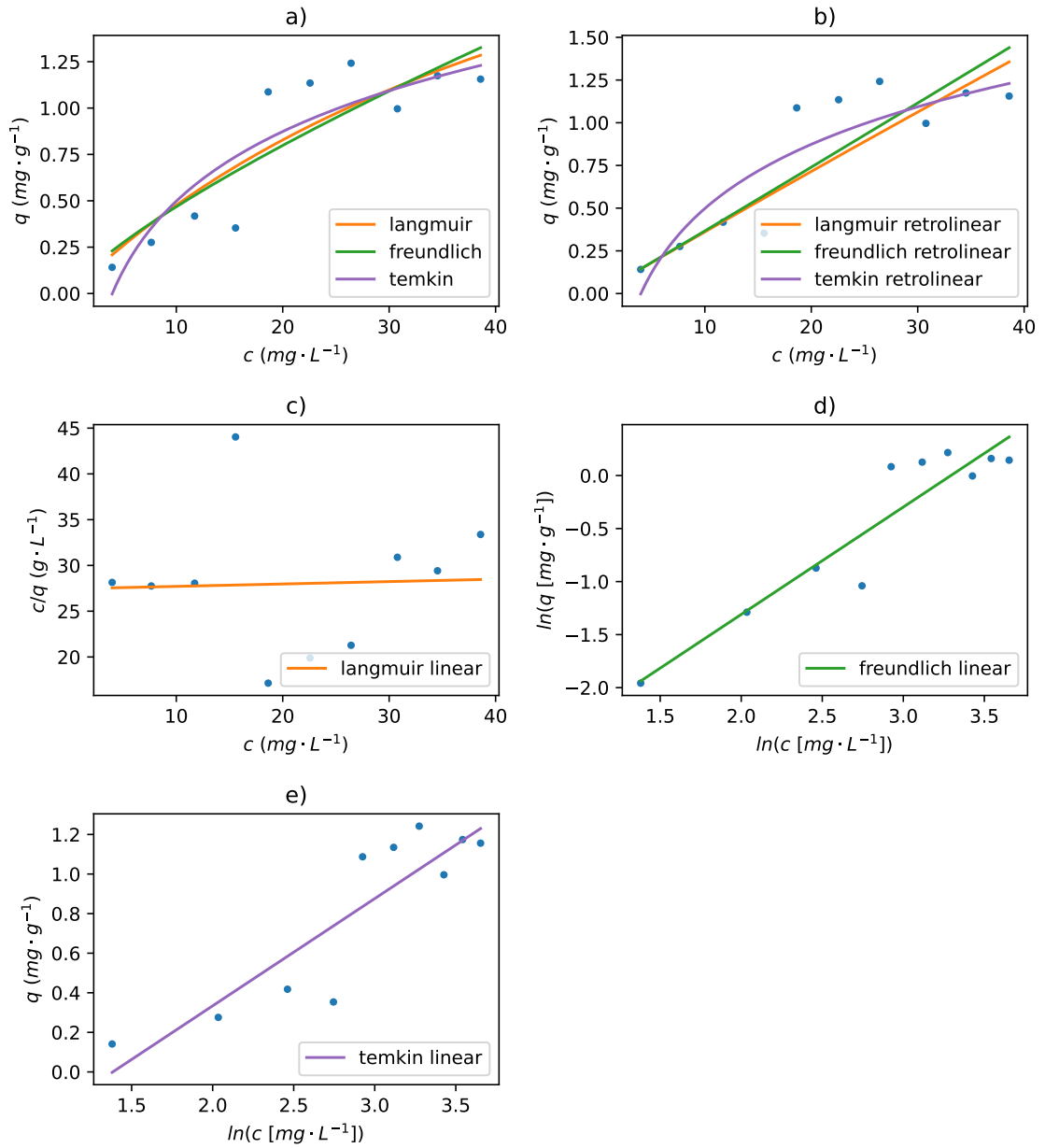
Figure A.3: Adsorption isotherms and their linearised forms for adsorption of Pb on smaller fraction PET (< 0,63 \mu\text{m} ) in seawater: a) adsorption isotherms constructed from non-linear fitting; b) adsorption isotherms constructed from linear fitting; c) Langmuir linear regression; d) Freundlich linear regression; e) Temkin linear regression.
