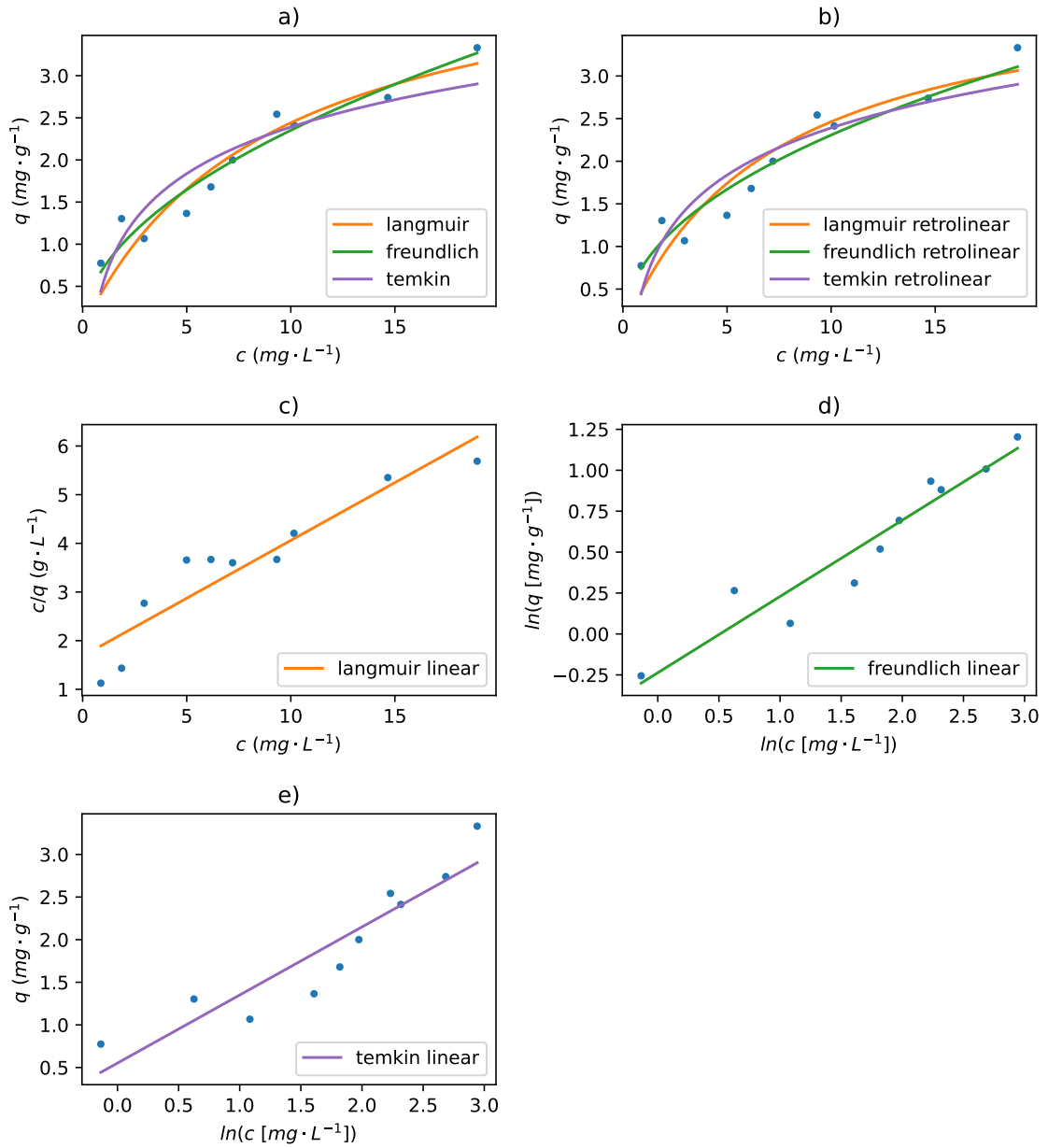
Figure A.18: Adsorption isotherms and their linearised forms for adsorption of Cd on smaller fraction PET (< 0,63 μm) in seawater: a) adsorption isotherms constructed from non-linear fitting; b) adsorption isotherms constructed from linear fitting; c) Langmuir linear regression; d) Freundlich linear regression; e) Temkin linear regression.
