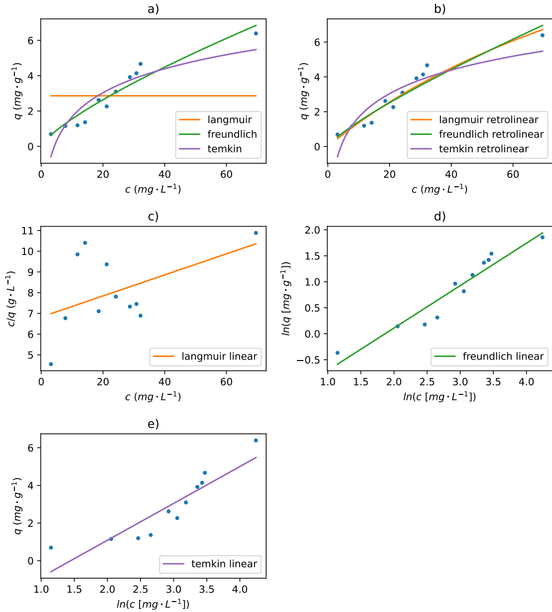
Figure A.1: Adsorption isotherms and their linearised forms for adsorption of Pb on smaller fraction PET (< 0,63 \mu\text{m} ) in freshwater: a) adsorption isotherms constructed from non-linear fitting; b) adsorption isotherms constructed from linear fitting; c) Langmuir linear regression; d) Freundlich linear regression; e) Temkin linear regression.
