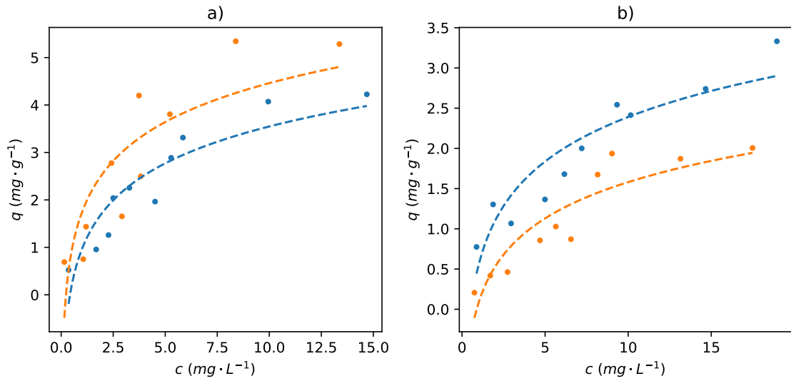
Figure 4.5: Measured data points of adsorption isotherms for Cd: a) fresh water, b) sea water; smaller PET fraction ( < 0,63 \mu\text{m} ) - blue, bigger PET fraction ( 0,63 \mu\text{m} - 1 \text{mm} ) - orange.
