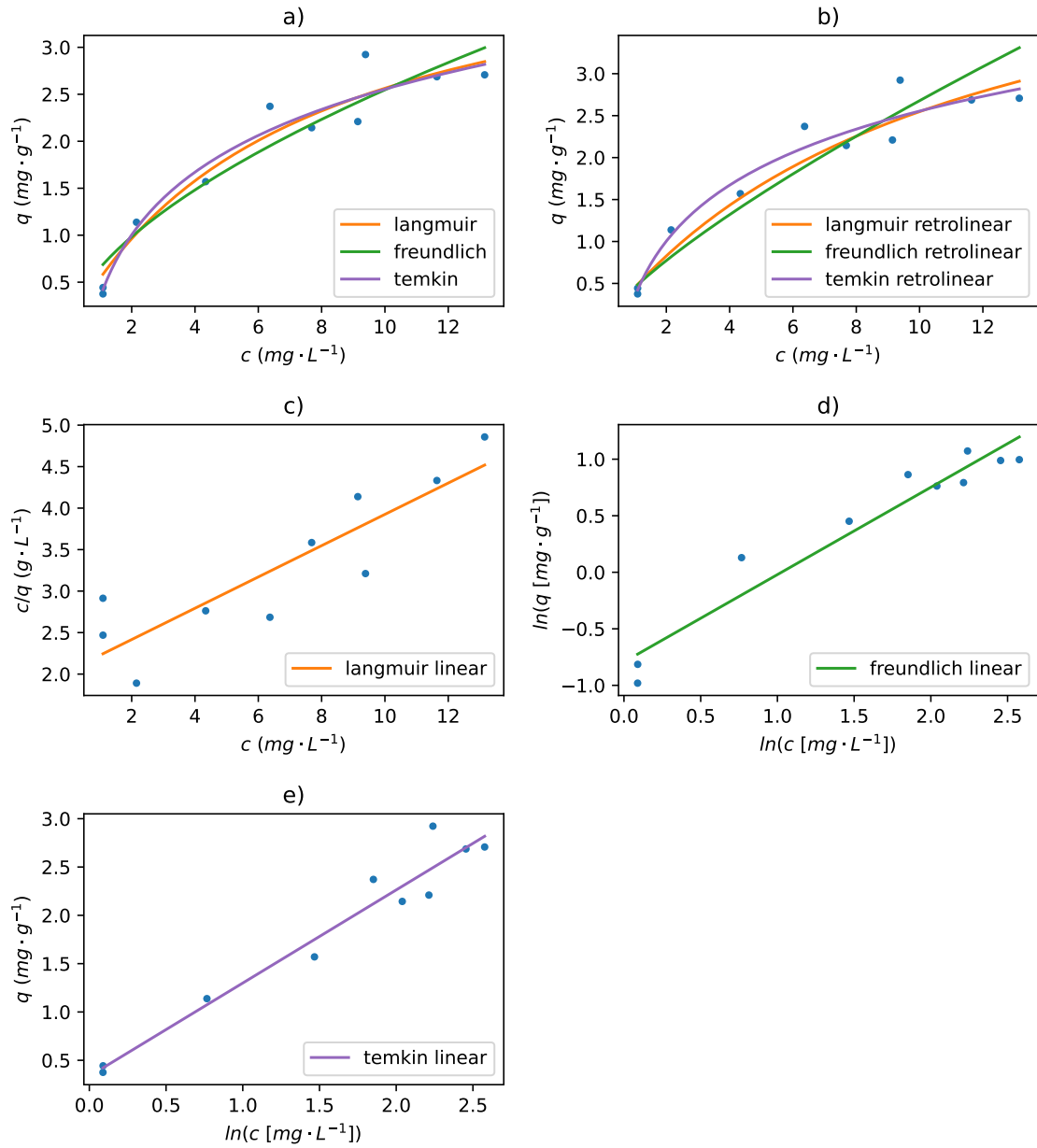
Figure A.15: Adsorption isotherms and their linearised forms for adsorption of Cu on bigger fraction PET (0,63 \mu\text{m} – 1 mm) in seawater: a) adsorption isotherms constructed from non-linear fitting; b) adsorption isotherms constructed from linear fitting; c) Langmuir linear regression; d) Freundlich linear regression; e) Temkin linear regression.
