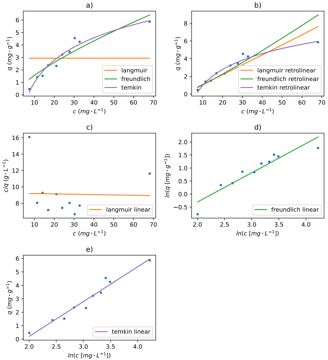
Figure A.2: Adsorption isotherms and their linearised forms for adsorption of Pb on bigger fraction PET ( 0,63 \mu m - 1 mm ) in freshwater: a) adsorption isotherms constructed from non-linear fitting; b) adsorption isotherms constructed from linear fitting; c) Langmuir linear regression; d) Freundlich linear regression; e) Temkin linear regression.
