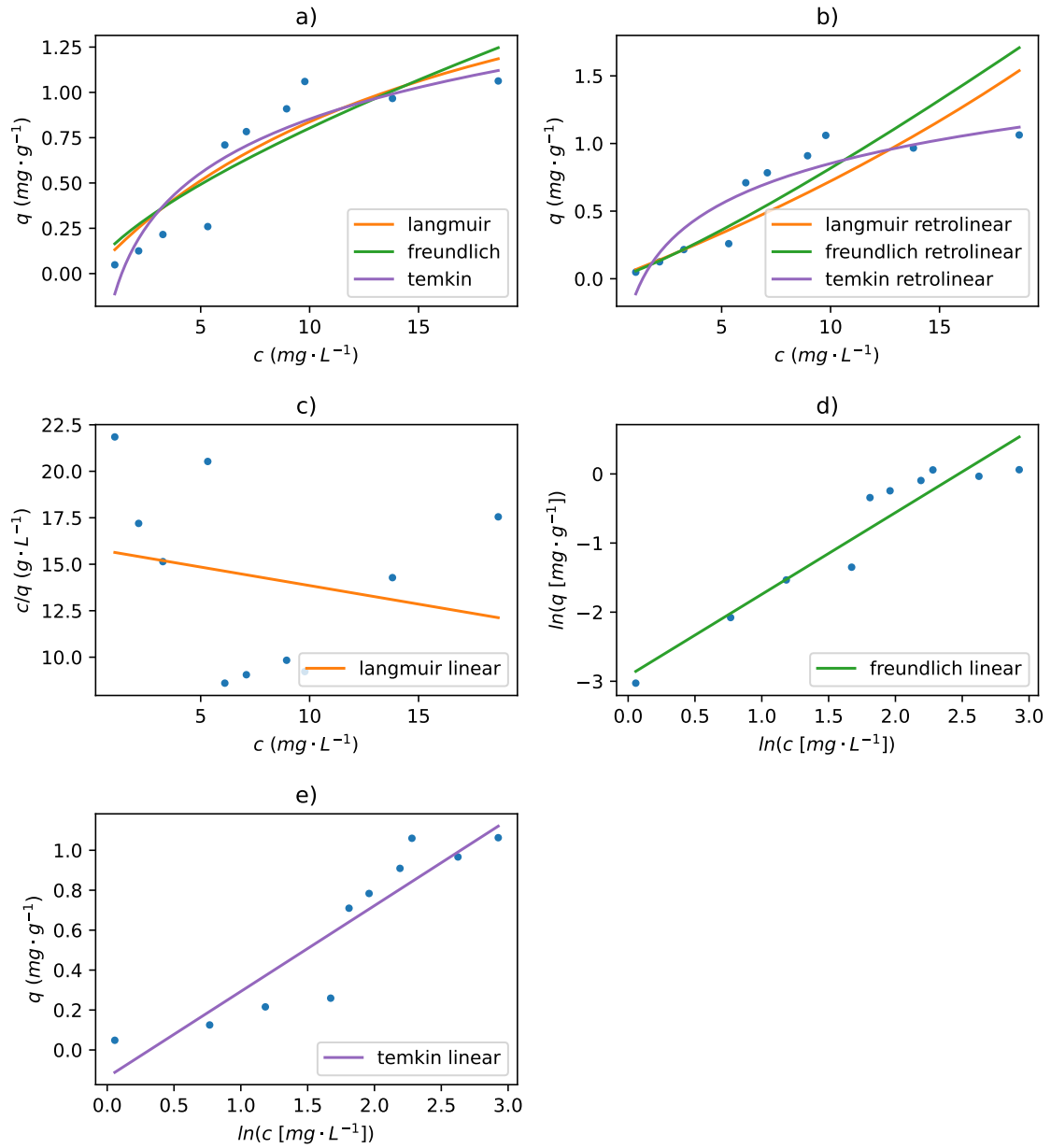
Figure A.7: Adsorption isotherms and their linearised forms for adsorption of Hg on smaller fraction PET (< 0,63 μm) in seawater: a) adsorption isotherms constructed from non-linear fitting; b) adsorption isotherms constructed from linear fitting; c) Langmuir linear regression; d) Freundlich linear regression; e) Temkin linear regression.
