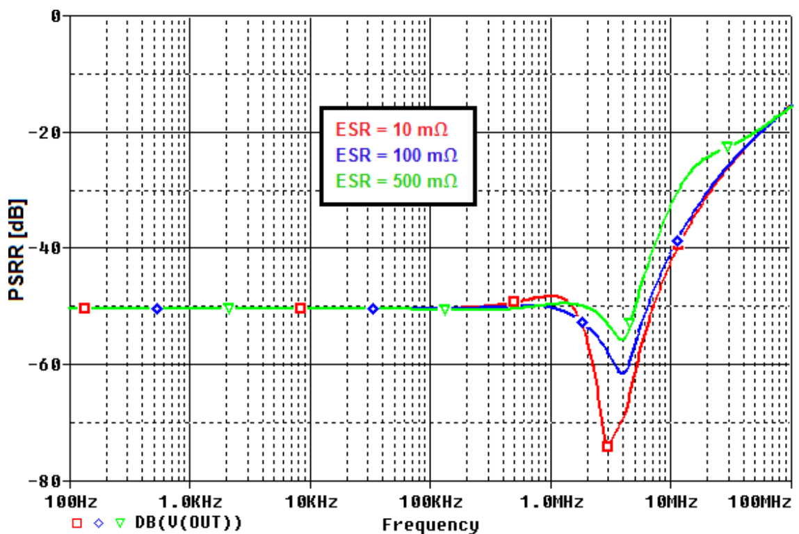
Obr. 4.15: PSRR LDO1 s proudovou vazbou 1 pro I_{ZATEZ} = 100 \text{ mA} , \text{ESR} = 10 \text{ m}\Omega , 100 \text{ m}\Omega , 500 \text{ m}\Omega .
