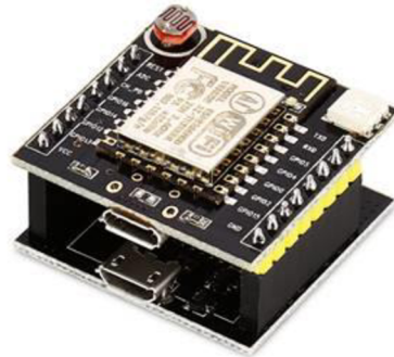
Figure 2.4: Witty Cloud development board.
